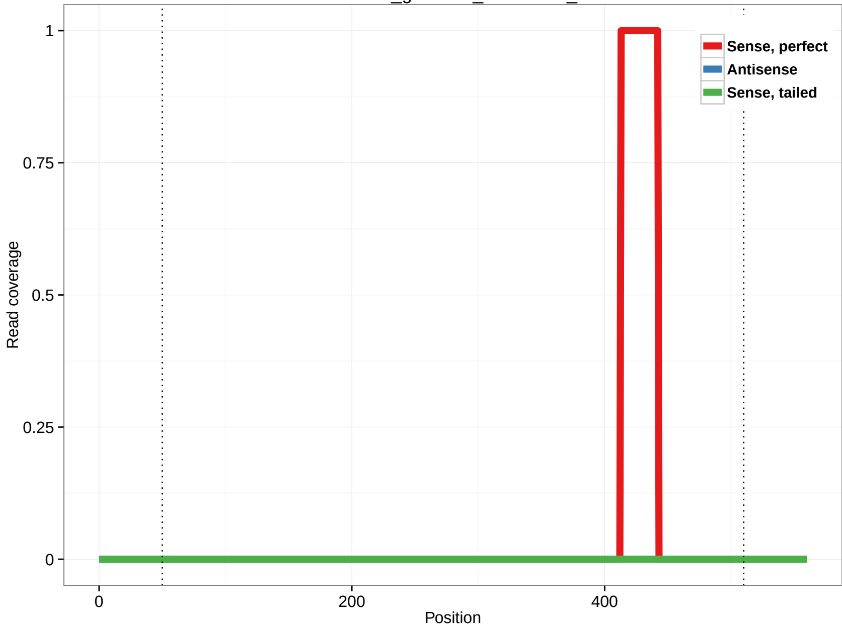
rheMac3_genscan_chr10.599_8
