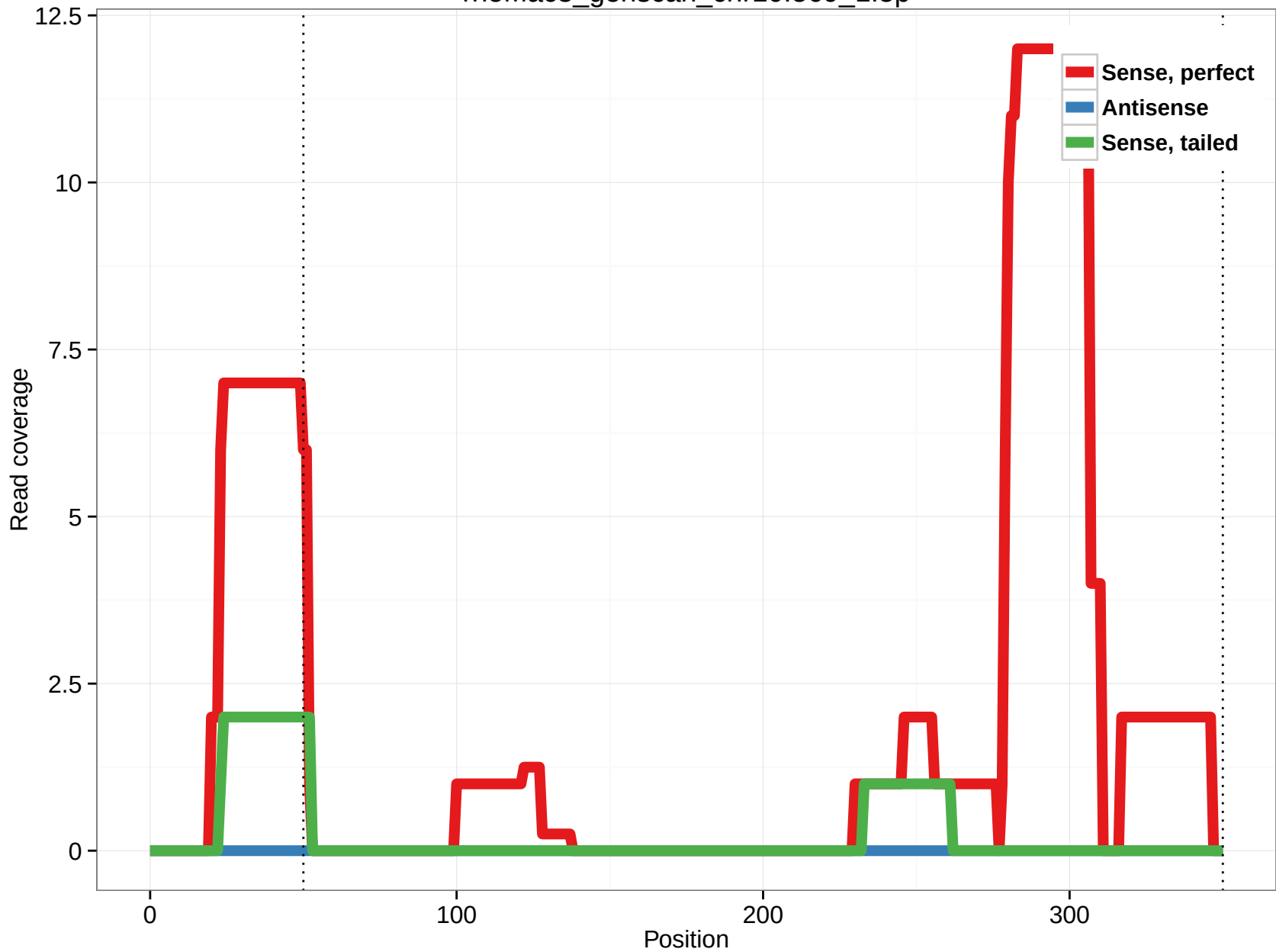
rheMac3_genscan_chr10.569_1.5p
