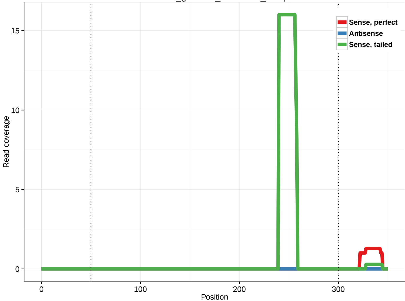
rheMac3_genscan_chr10.565_30.3p
