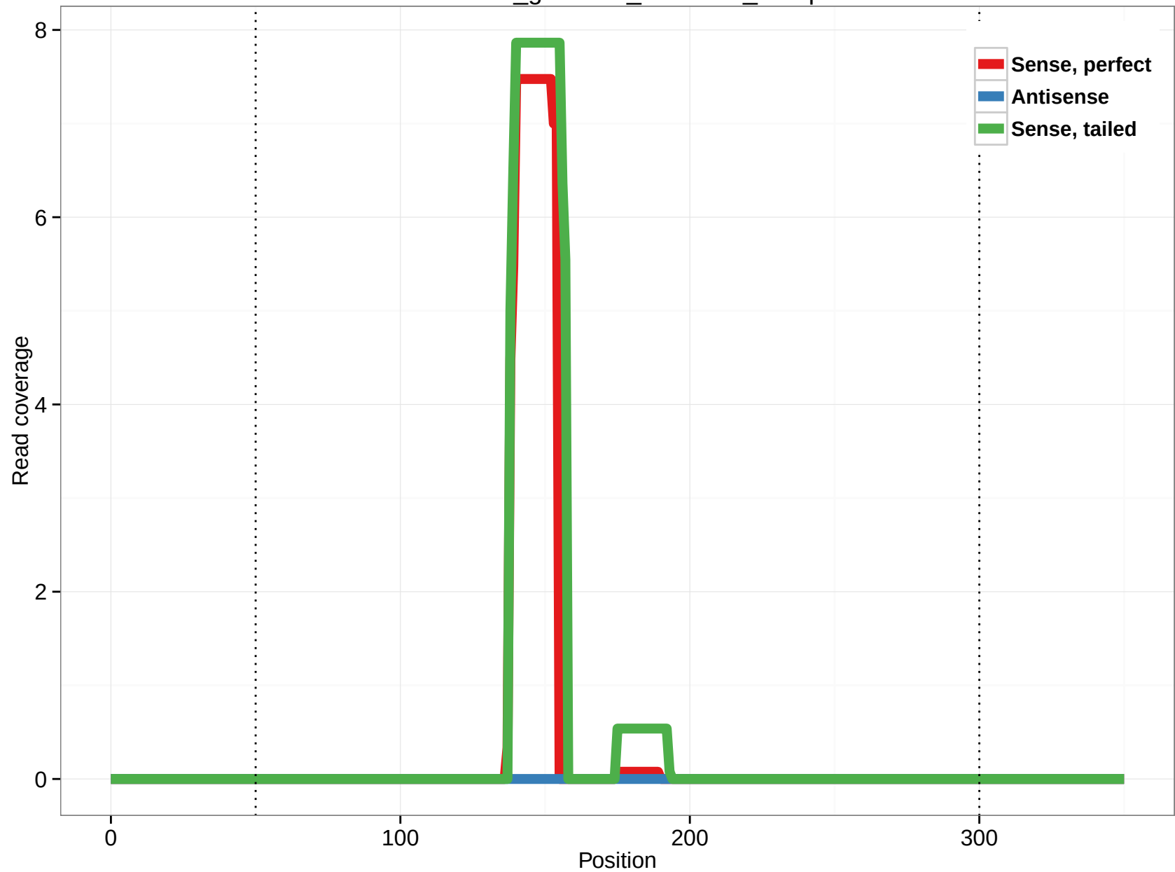
rheMac3_genscan_chr10.45_23.5p
