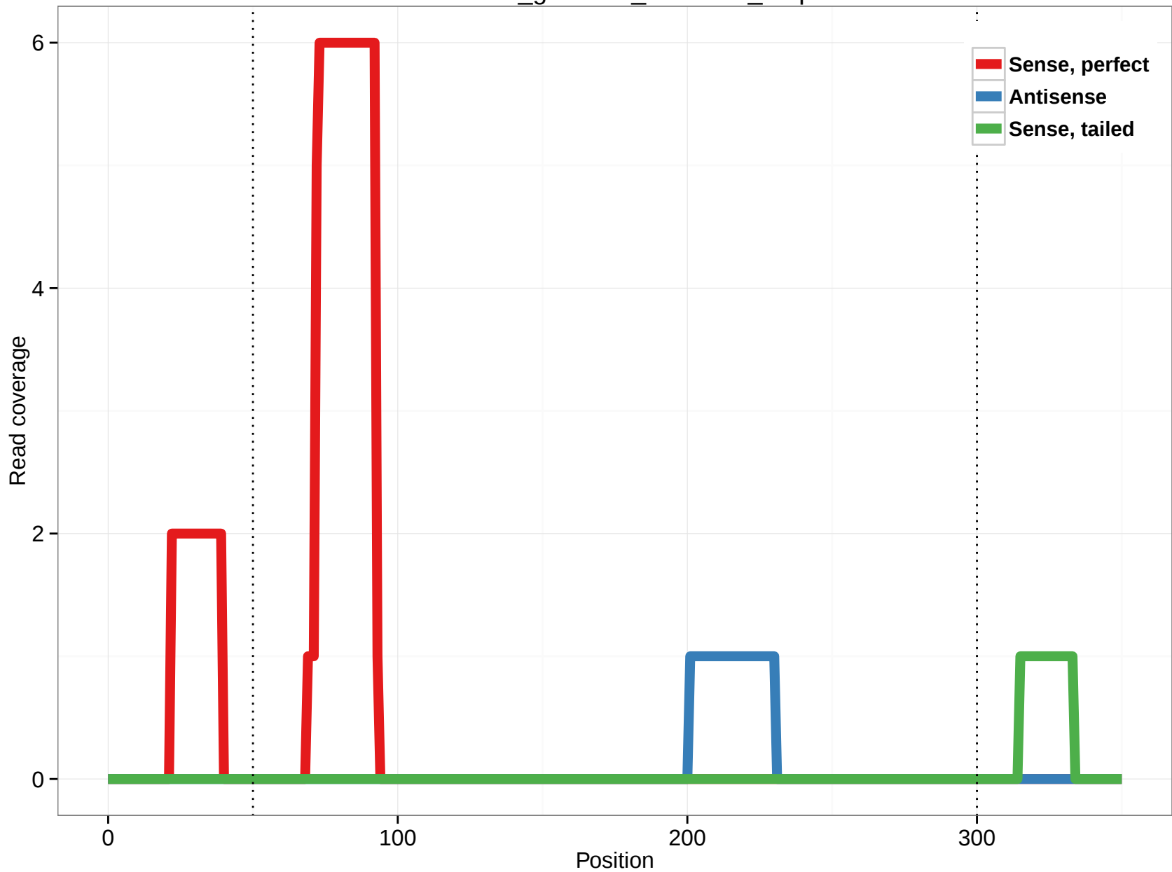
rheMac3_genscan_chr10.41_5.5p
