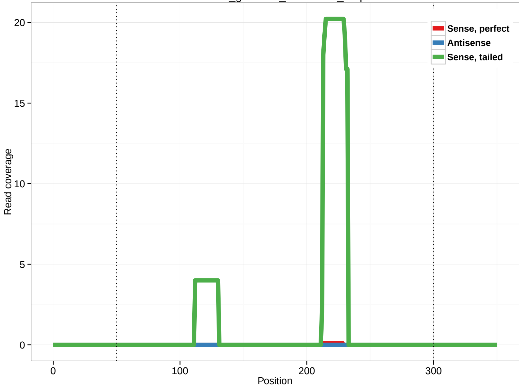
rheMac3_genscan_chr10.370_2.5p
