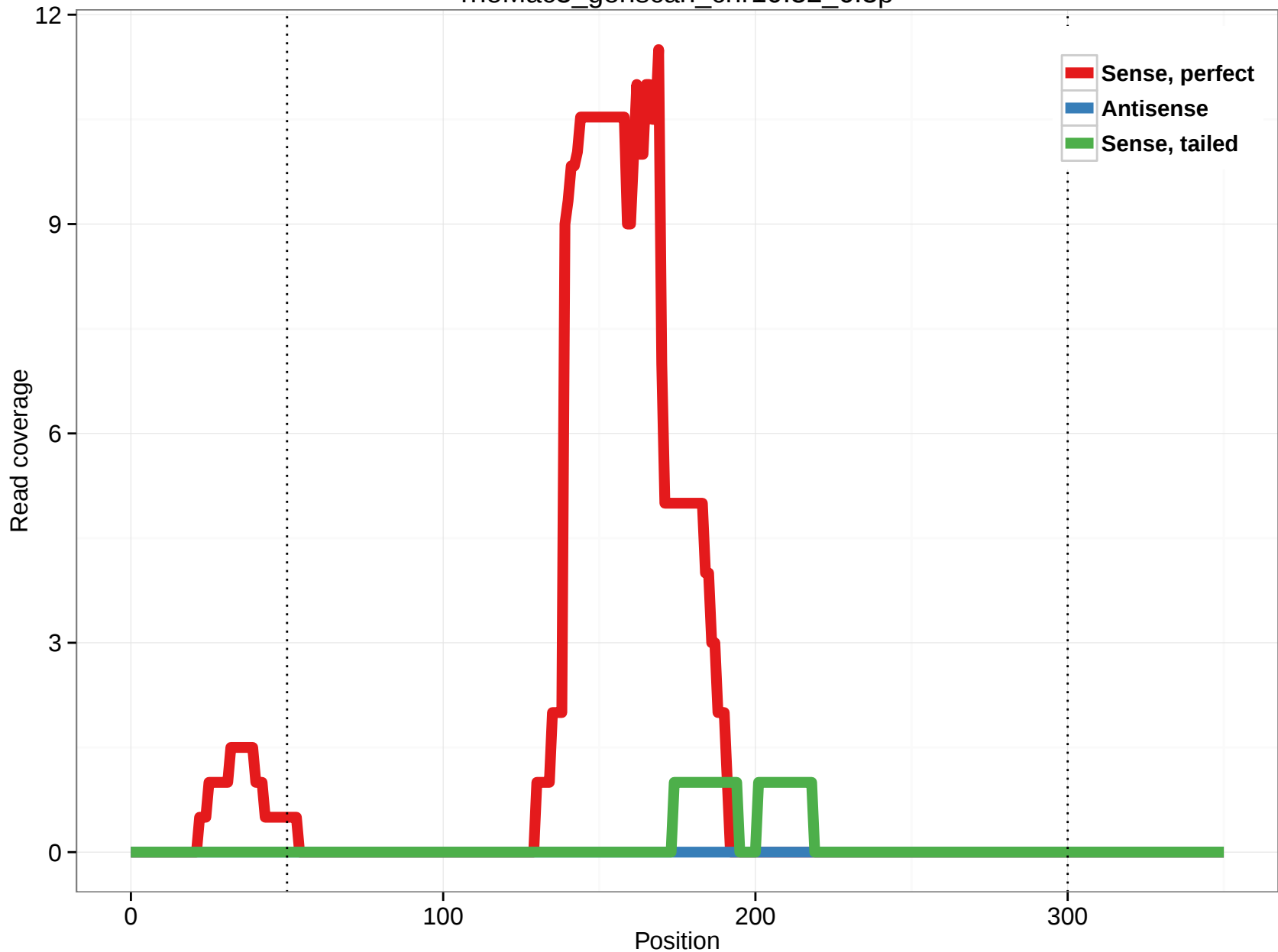
rheMac3_genscan_chr10.32_6.3p
