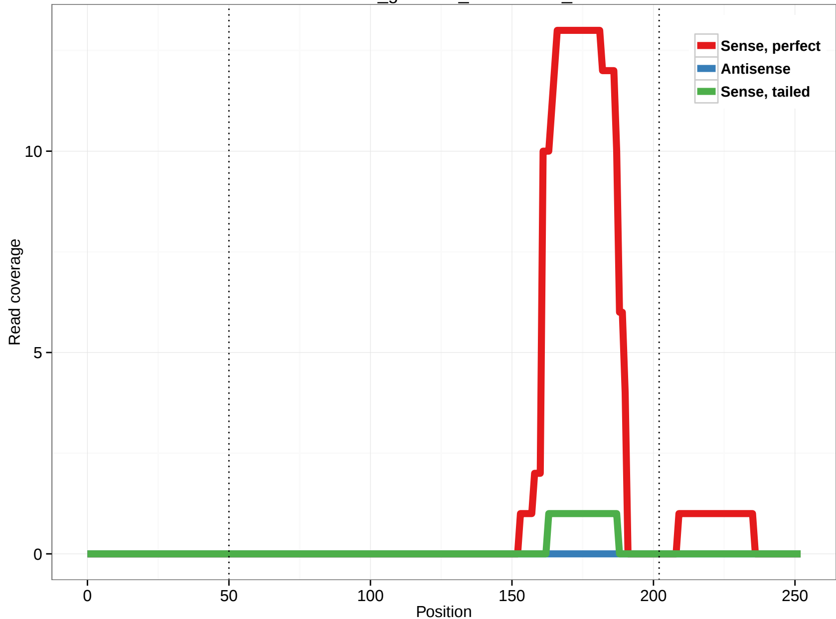
rheMac3_genscan_chr10.2306_5
