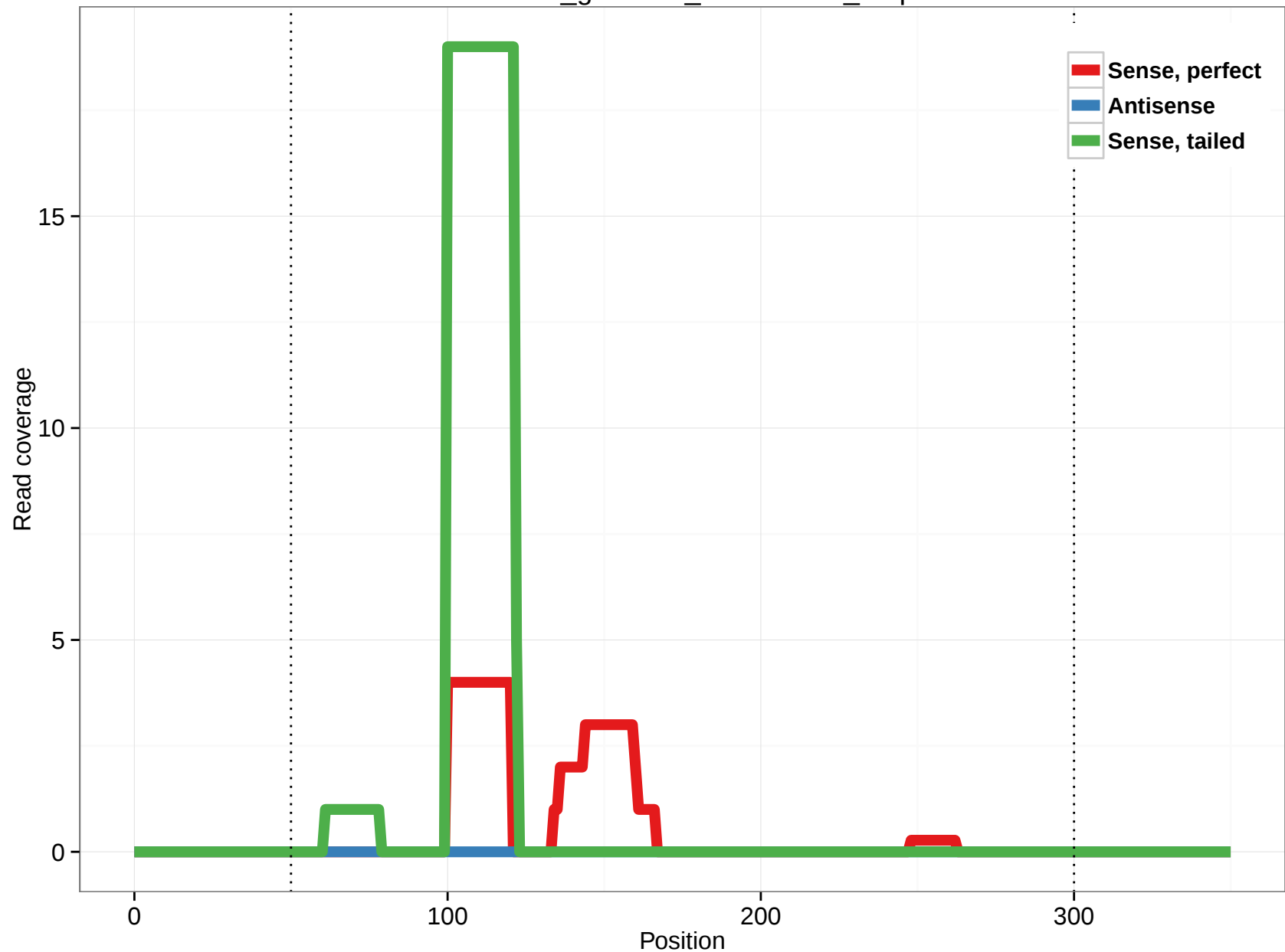
rheMac3_genscan_chr10.2305_8.5p
