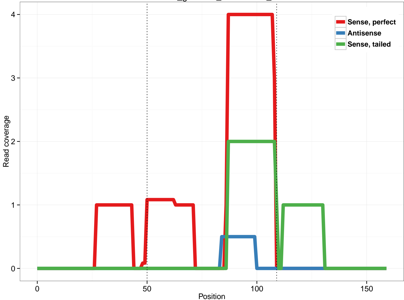
rheMac3_genscan_chr10.2301_39
