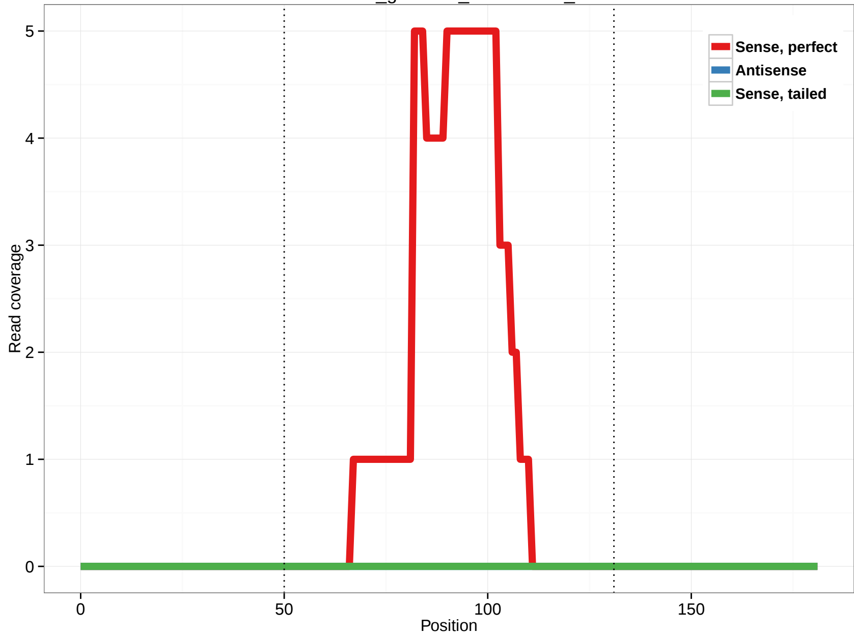
rheMac3_genscan_chr10.2301_37
