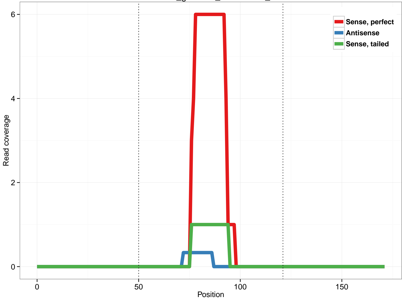
rheMac3_genscan_chr10.2297_25
