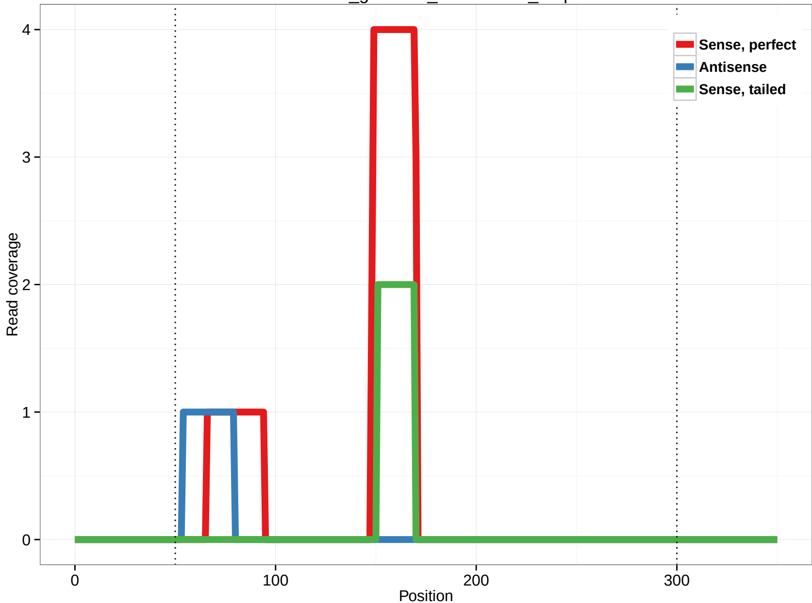
rheMac3_genscan_chr10.2296_0.5p
