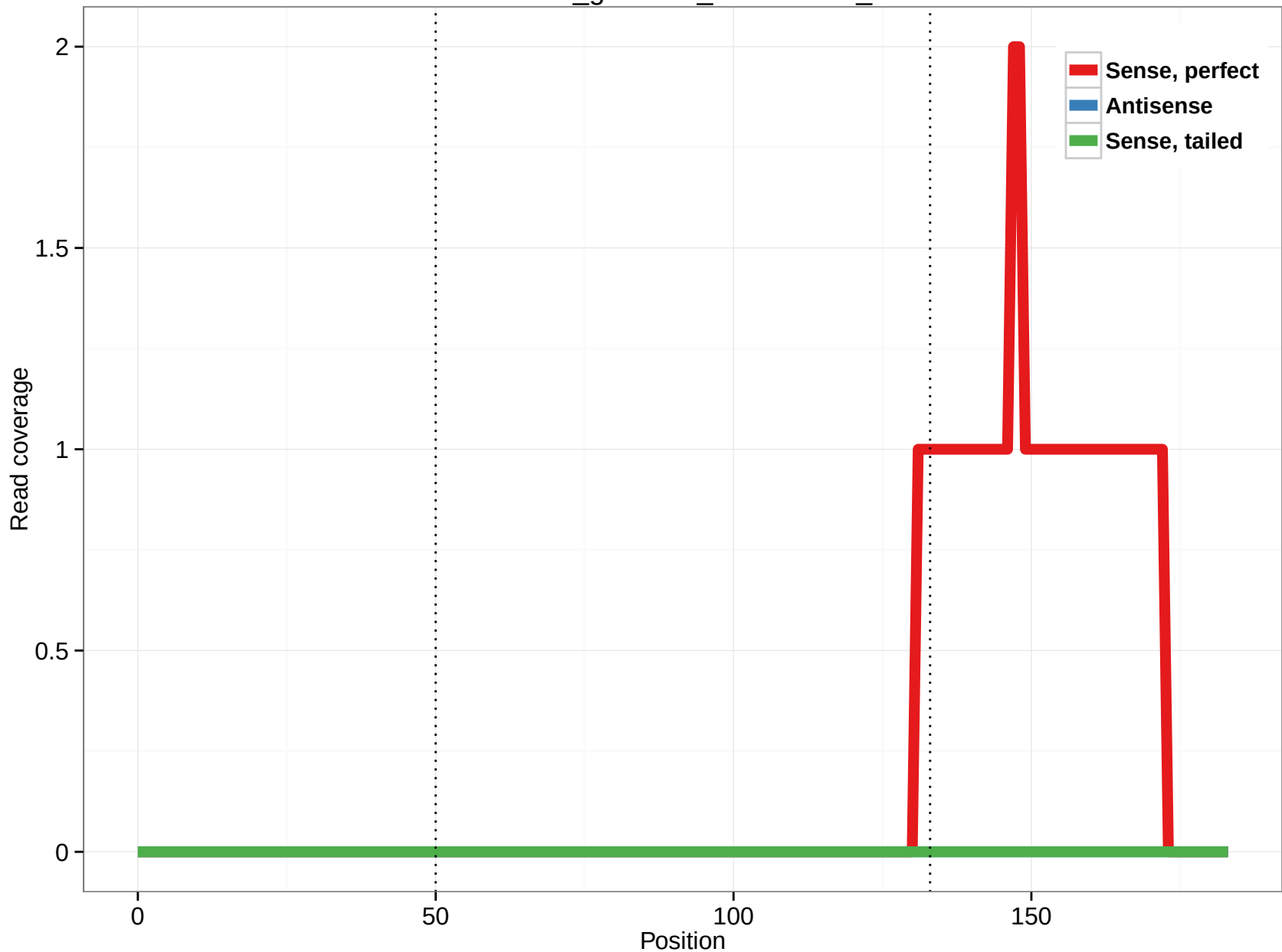
rheMac3_genscan_chr10.2295_37
