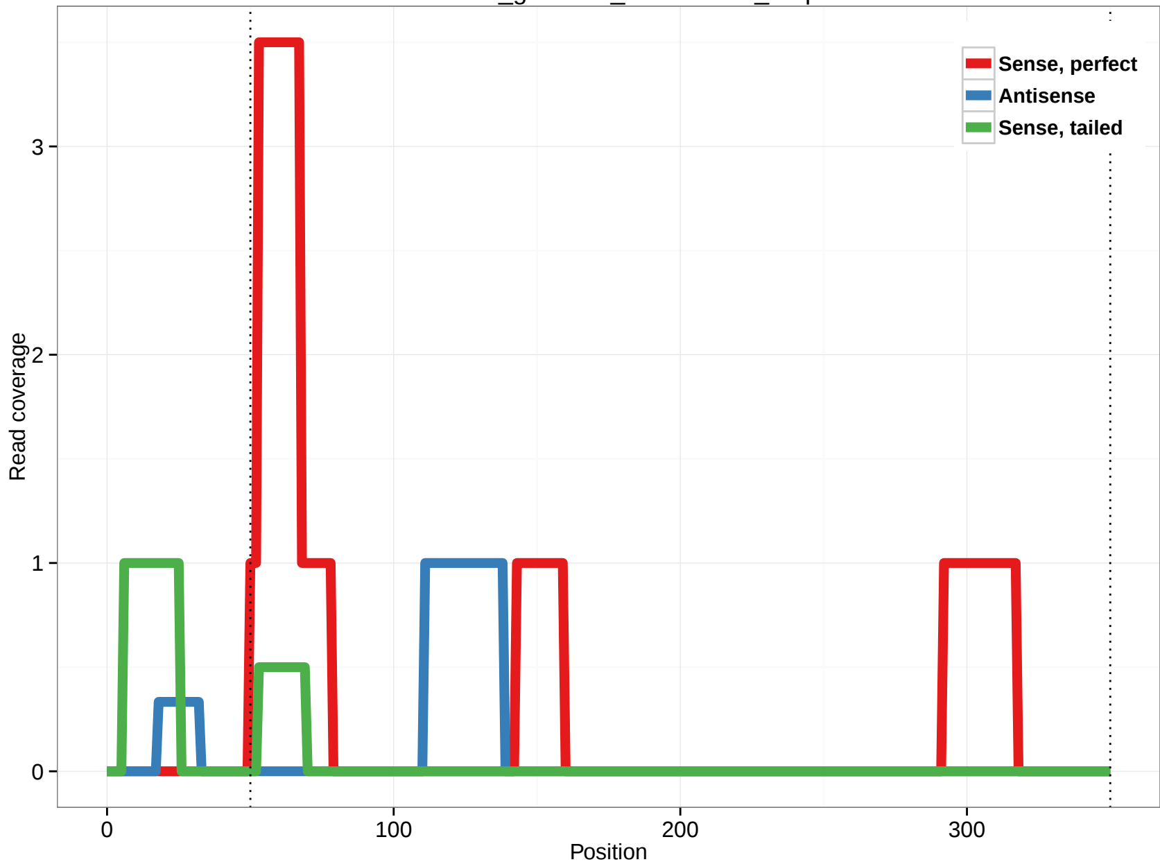
rheMac3_genscan_chr10.2270_6.5p
