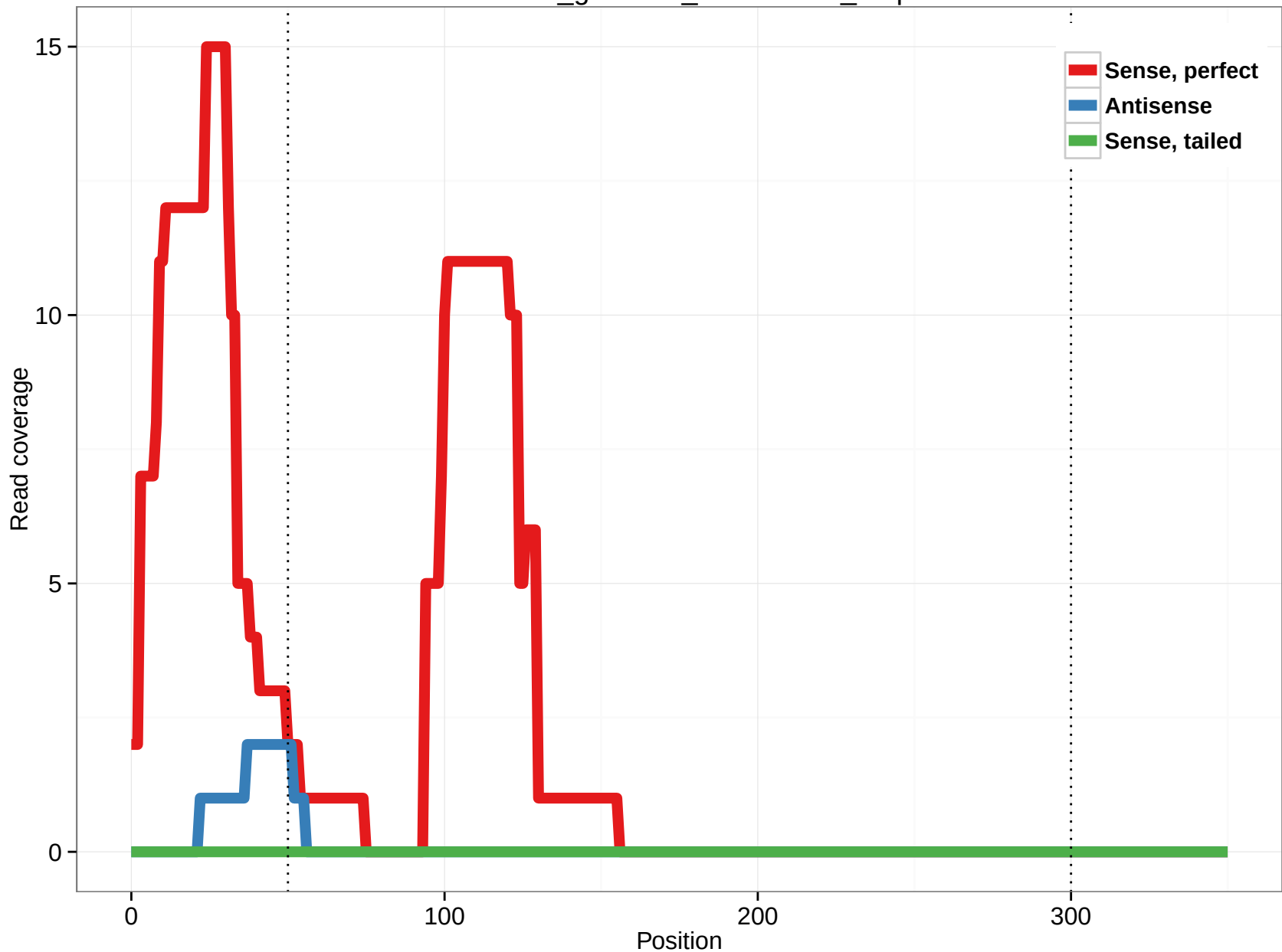
rheMac3_genscan_chr10.2227_0.3p
