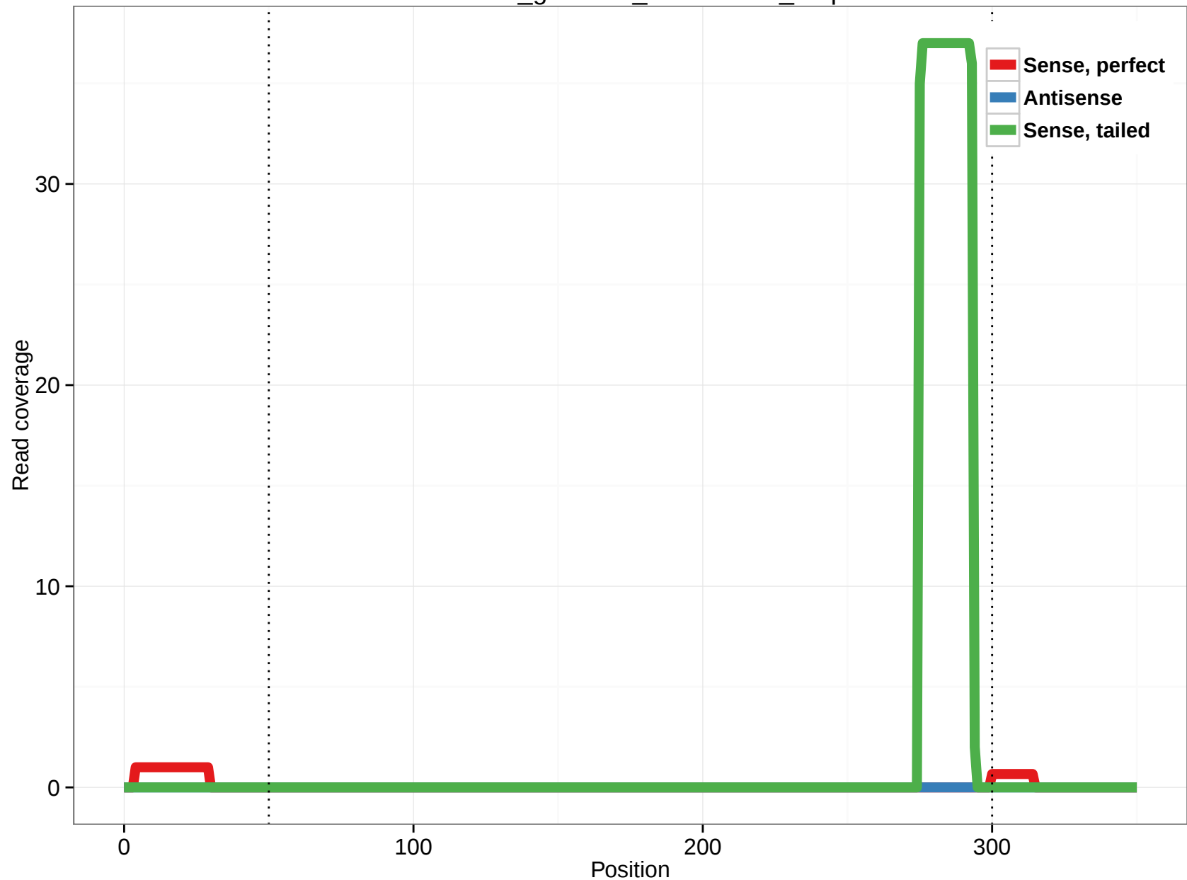
rheMac3_genscan_chr10.2166_2.5p
