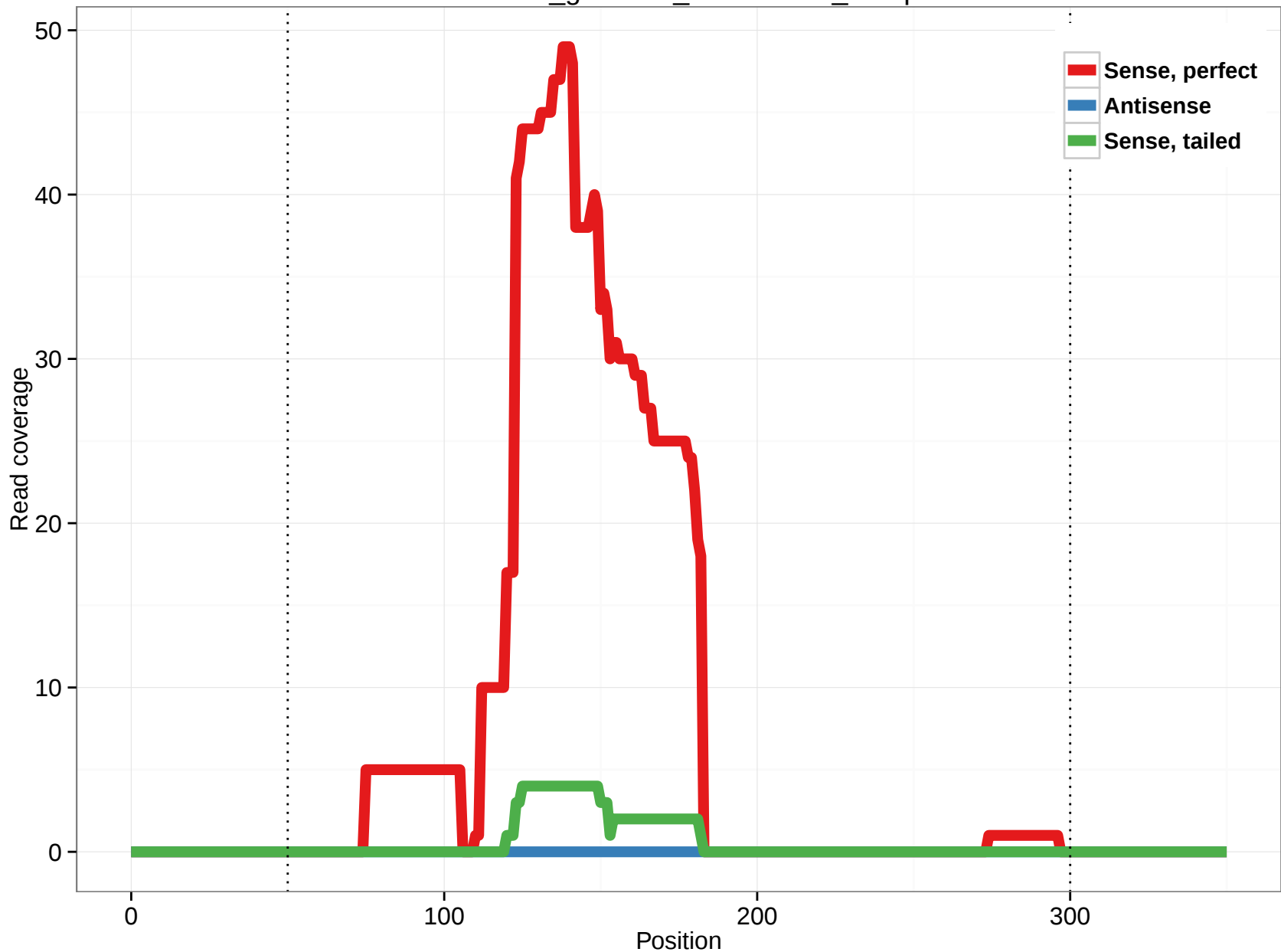
rheMac3_genscan_chr10.2100_14.3p
