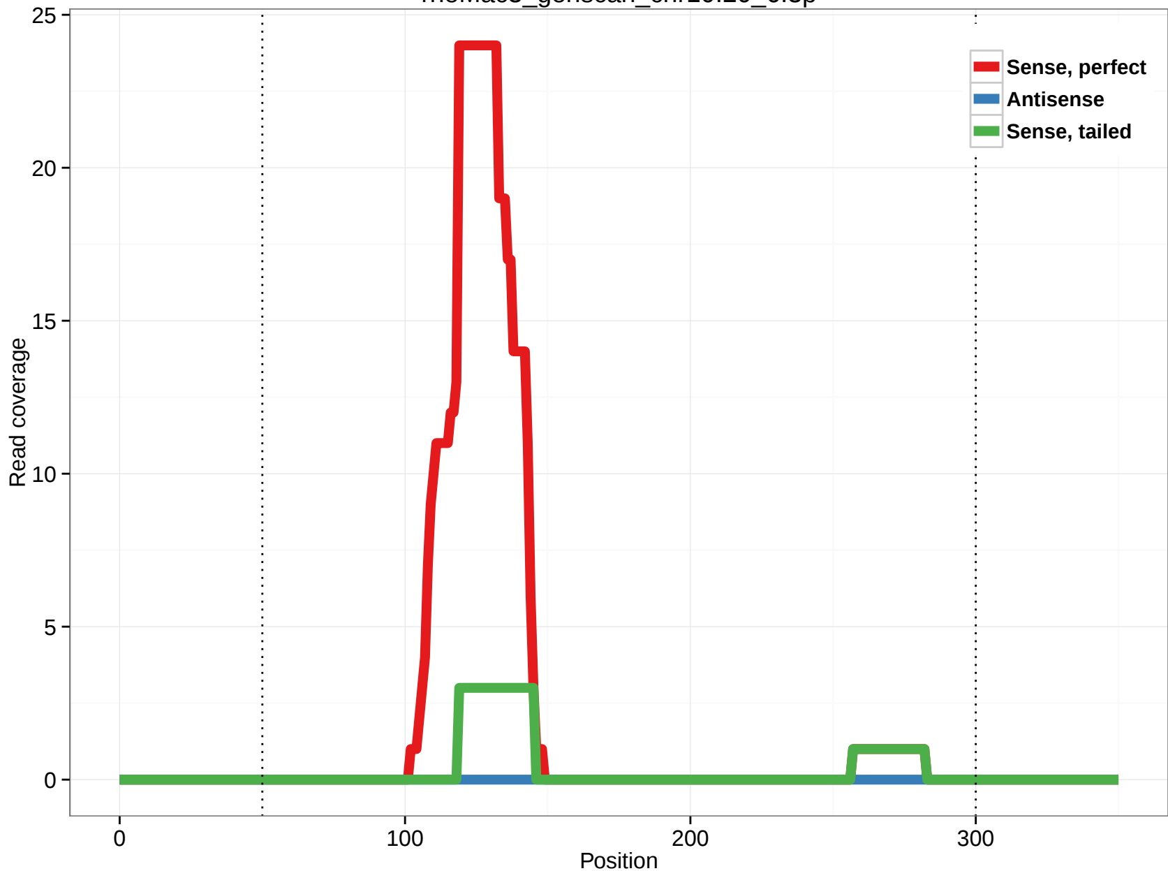
rheMac3_genscan_chr10.20_6.3p
