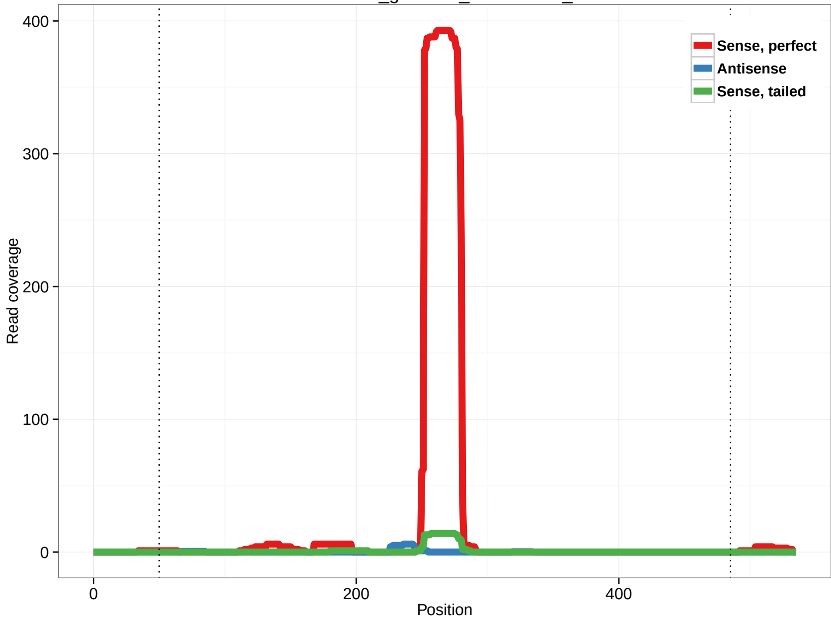
rheMac3_genscan_chr10.2005_2
