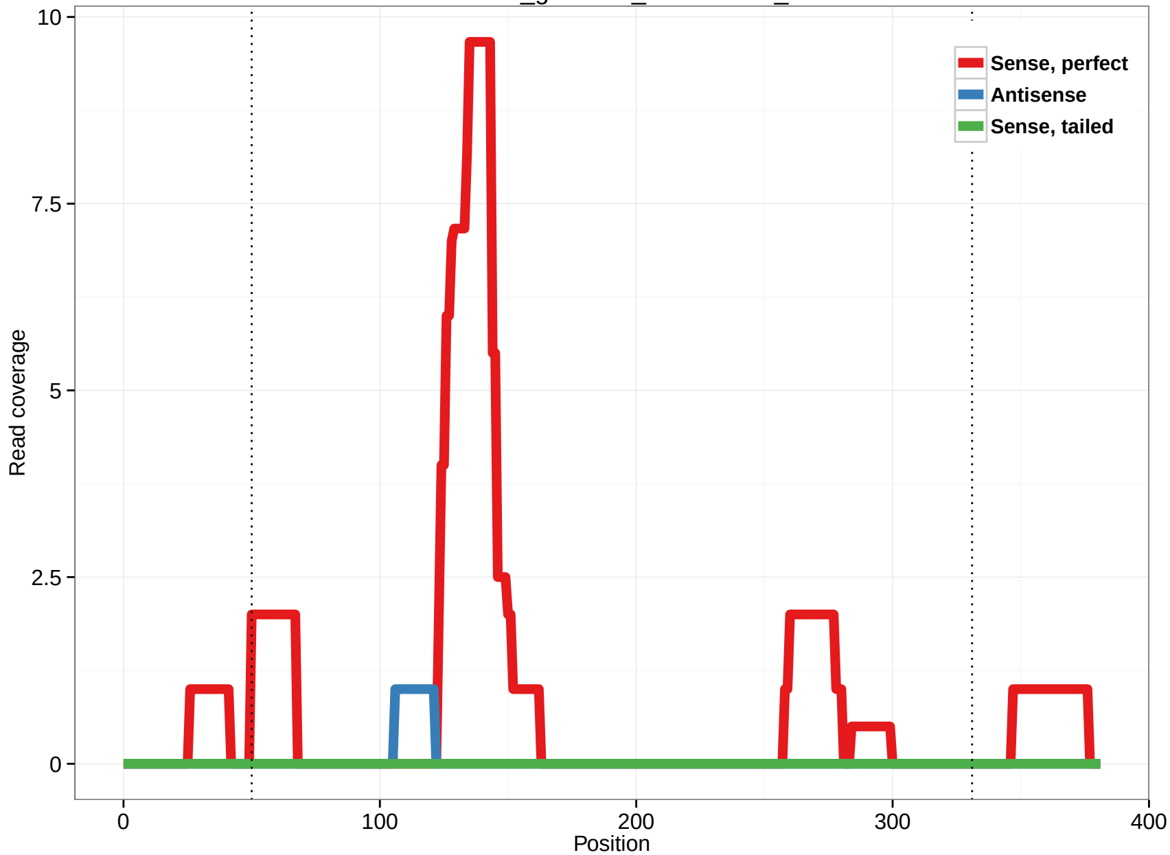
rheMac3_genscan_chr10.1970_0
