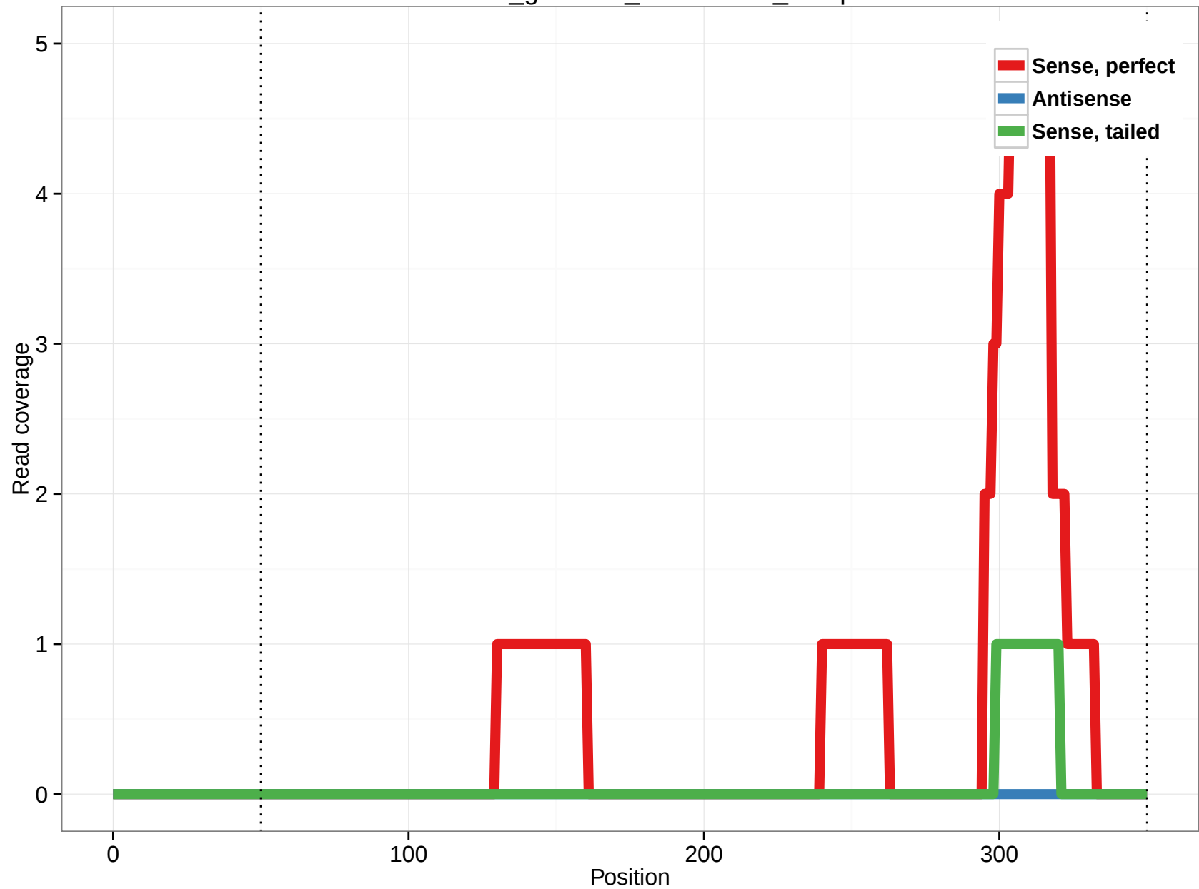
rheMac3_genscan_chr10.1962_13.5p
