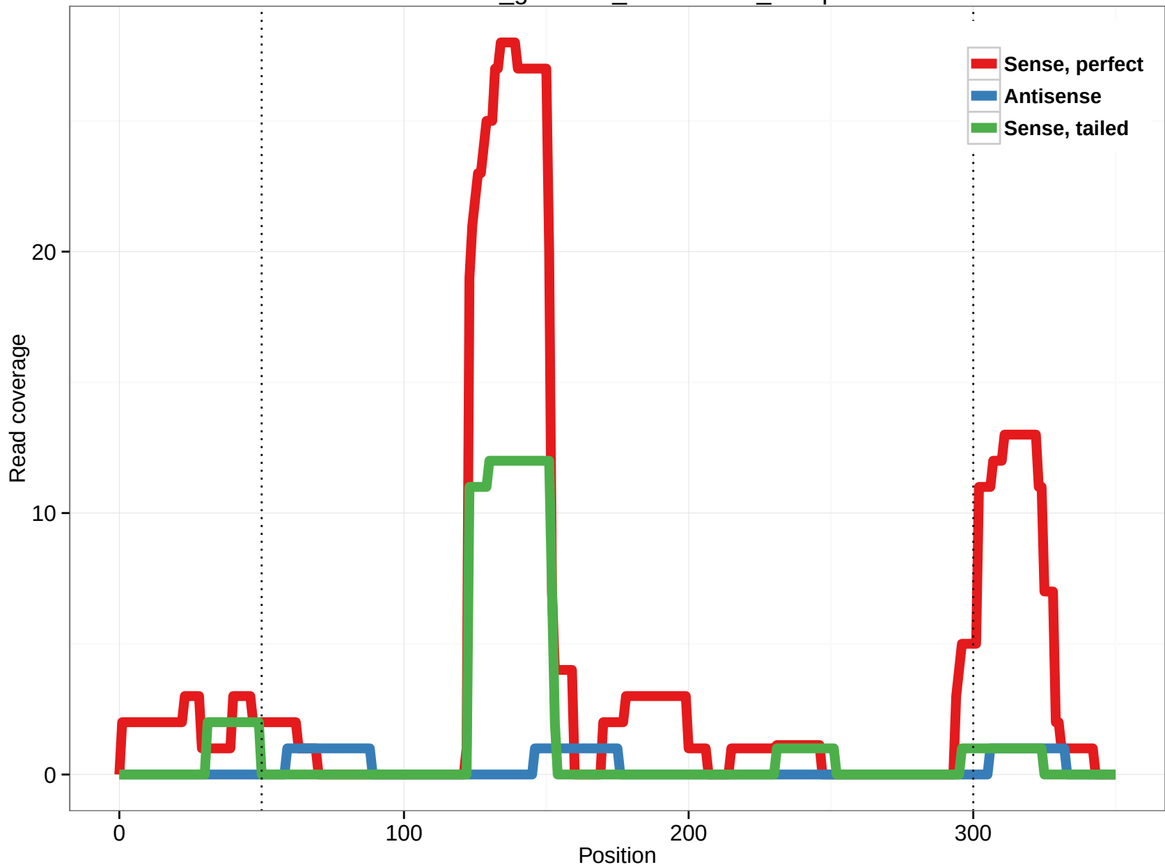
rheMac3_genscan_chr10.1931_10.5p
