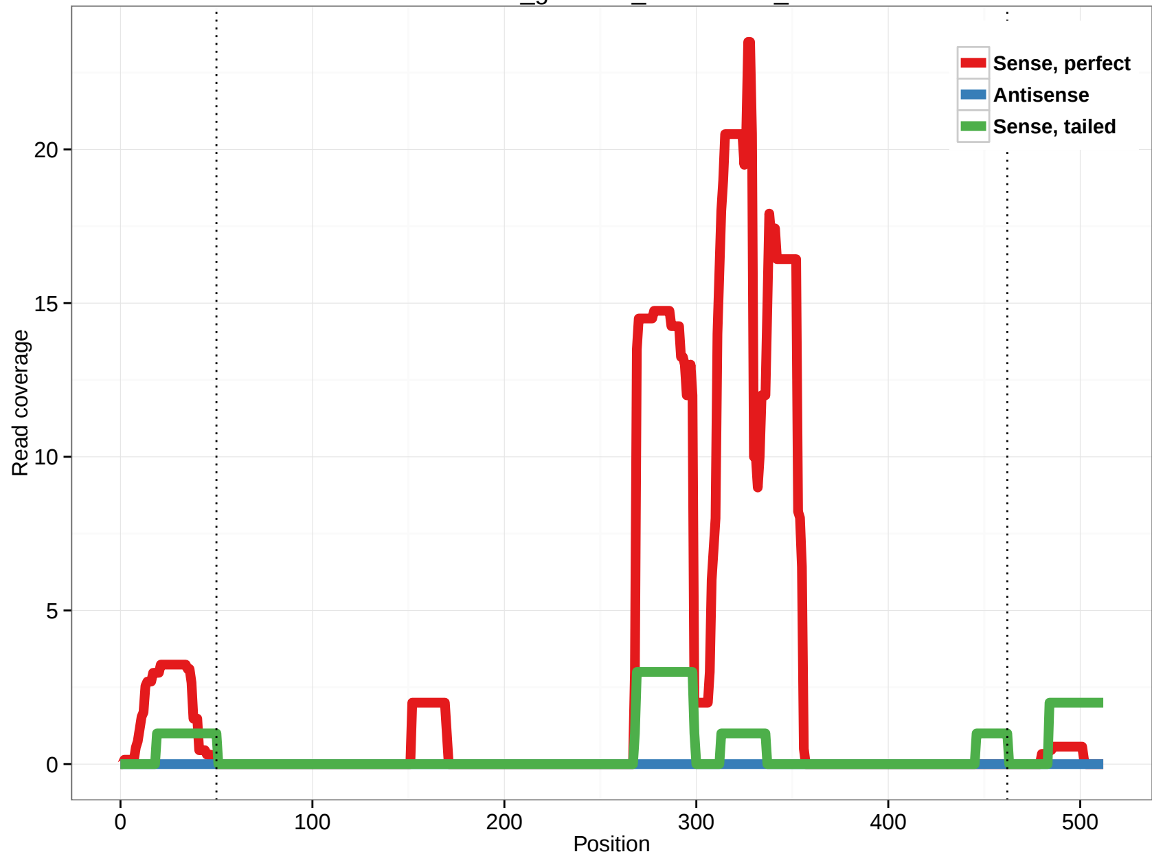
rheMac3_genscan_chr10.1920_6
