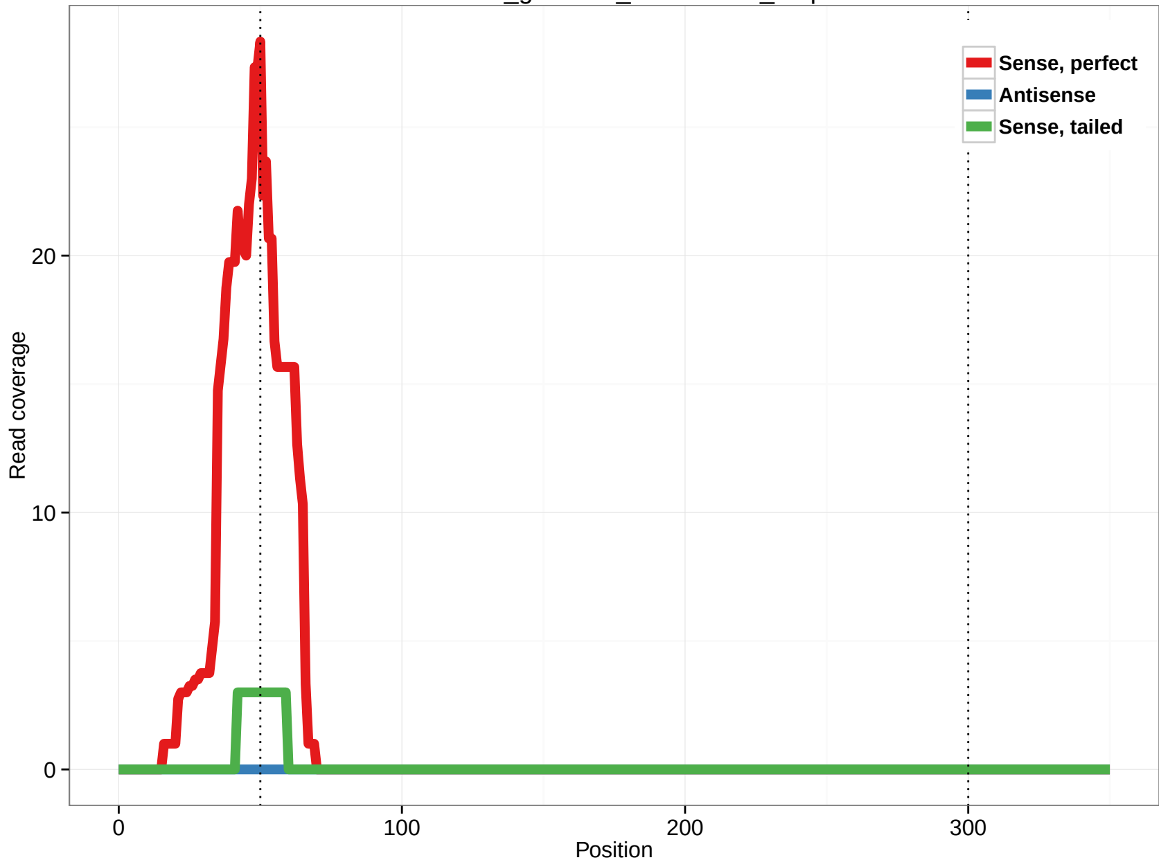
rheMac3_genscan_chr10.1920_0.5p
