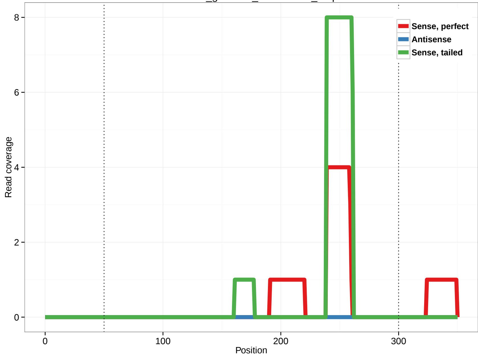
rheMac3_genscan_chr10.1918_2.3p
