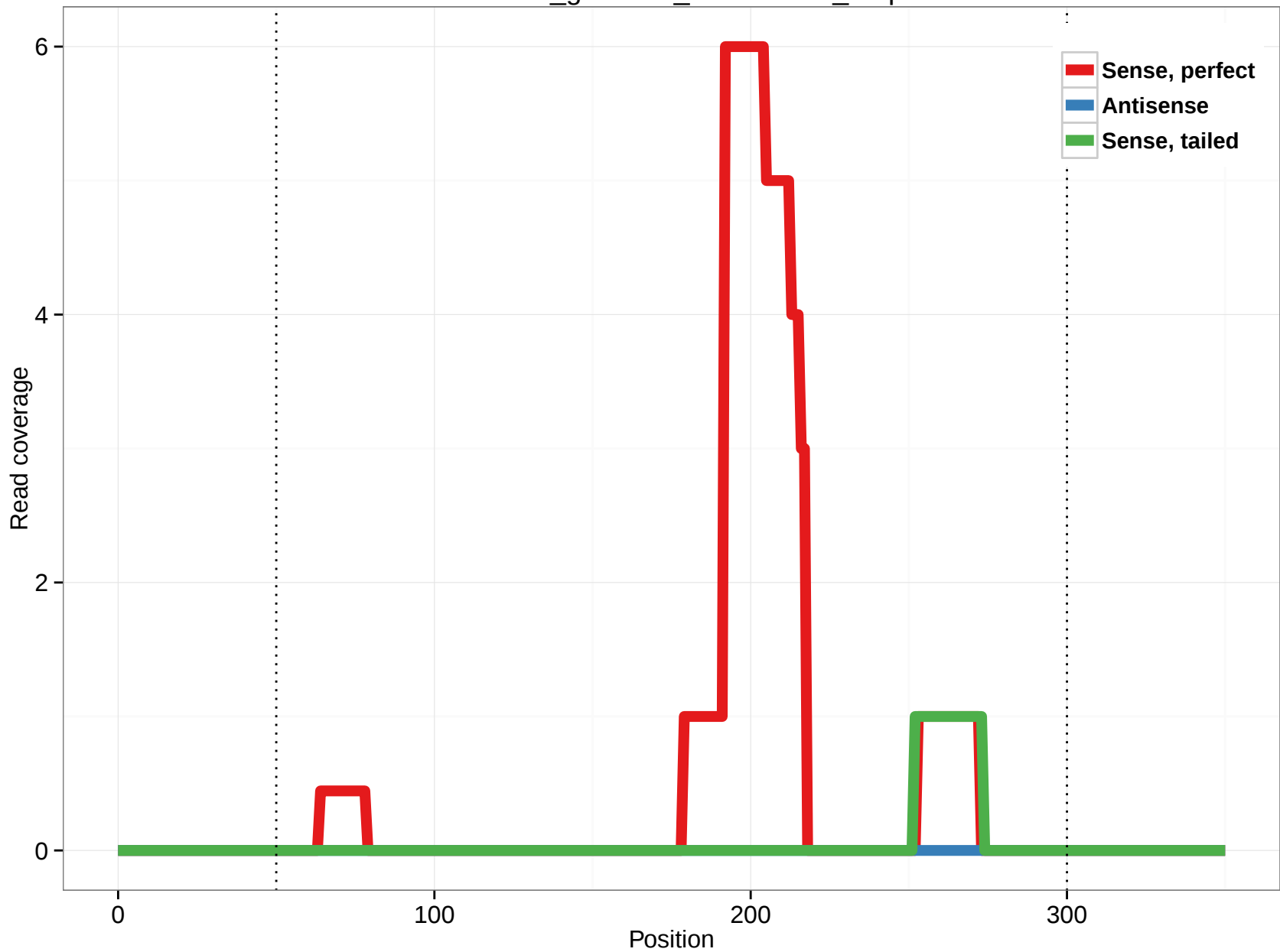
rheMac3_genscan_chr10.1914_1.3p
