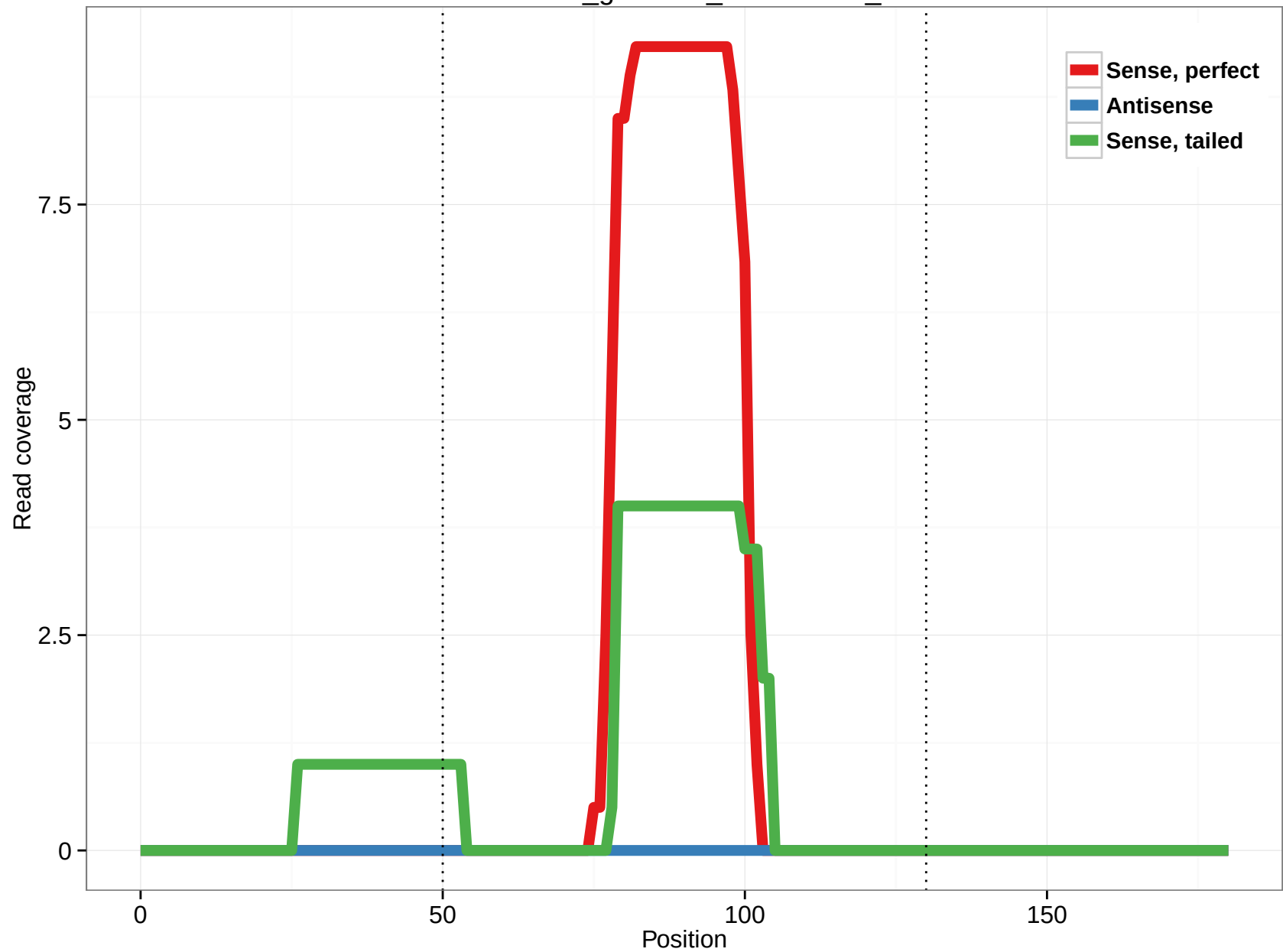
rheMac3_genscan_chr10.1891_2
