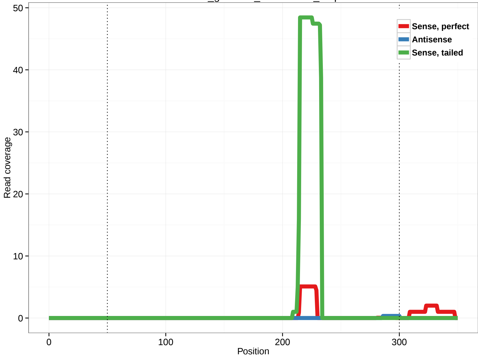
rheMac3_genscan_chr10.1888_7.3p
