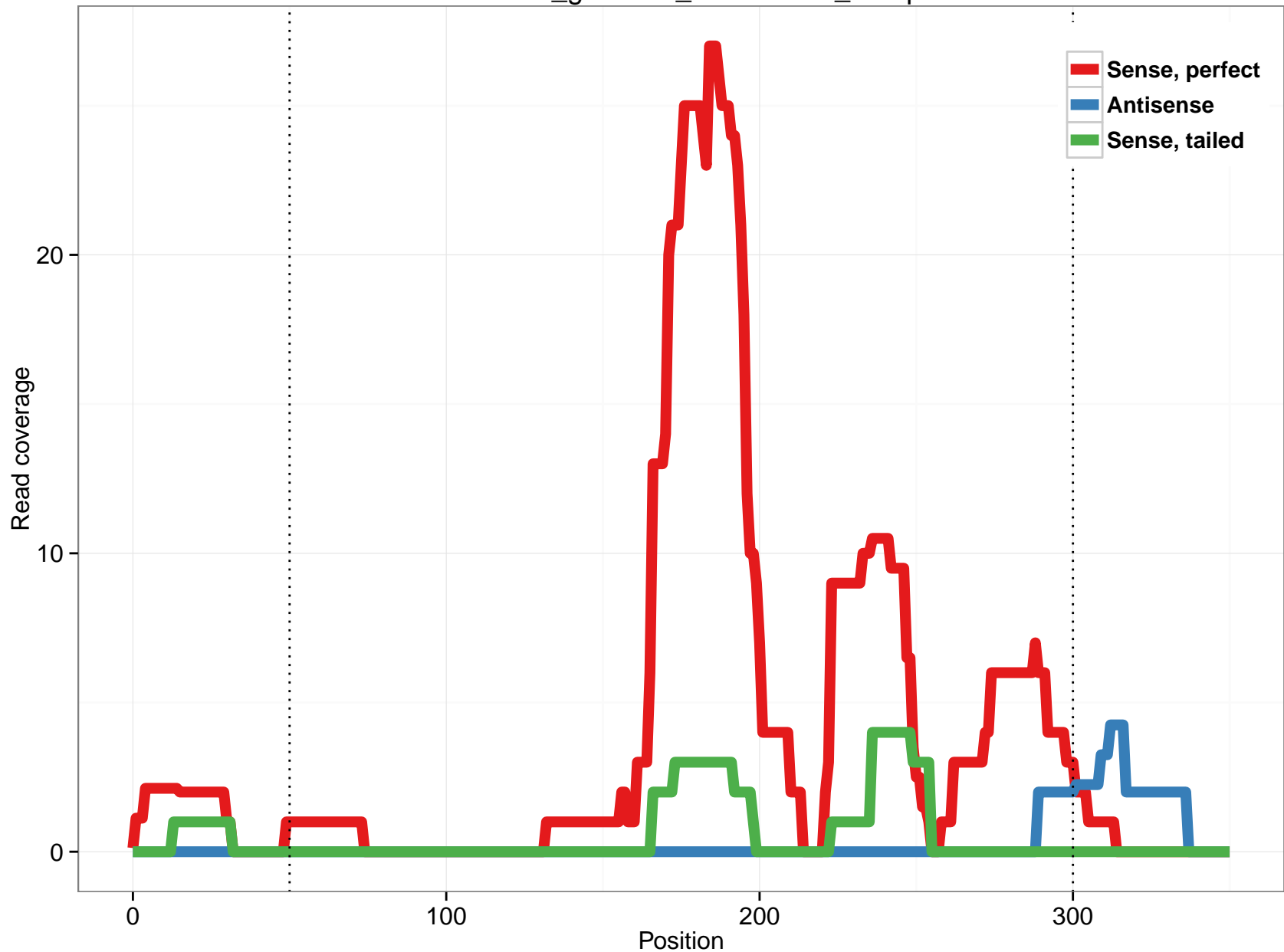
rheMac3_genscan_chr10.1888_12.3p
