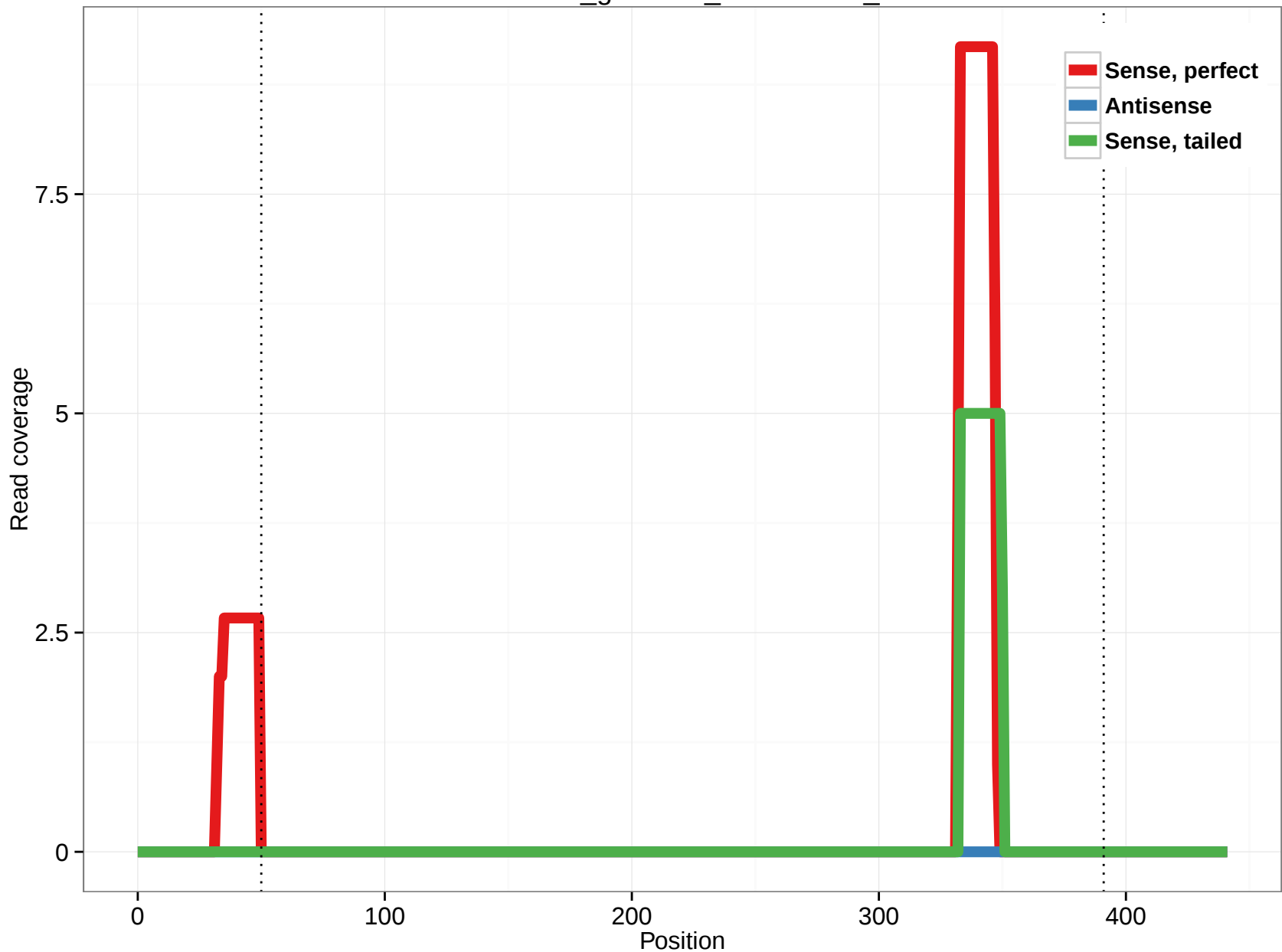
rheMac3_genscan_chr10.1879_2
