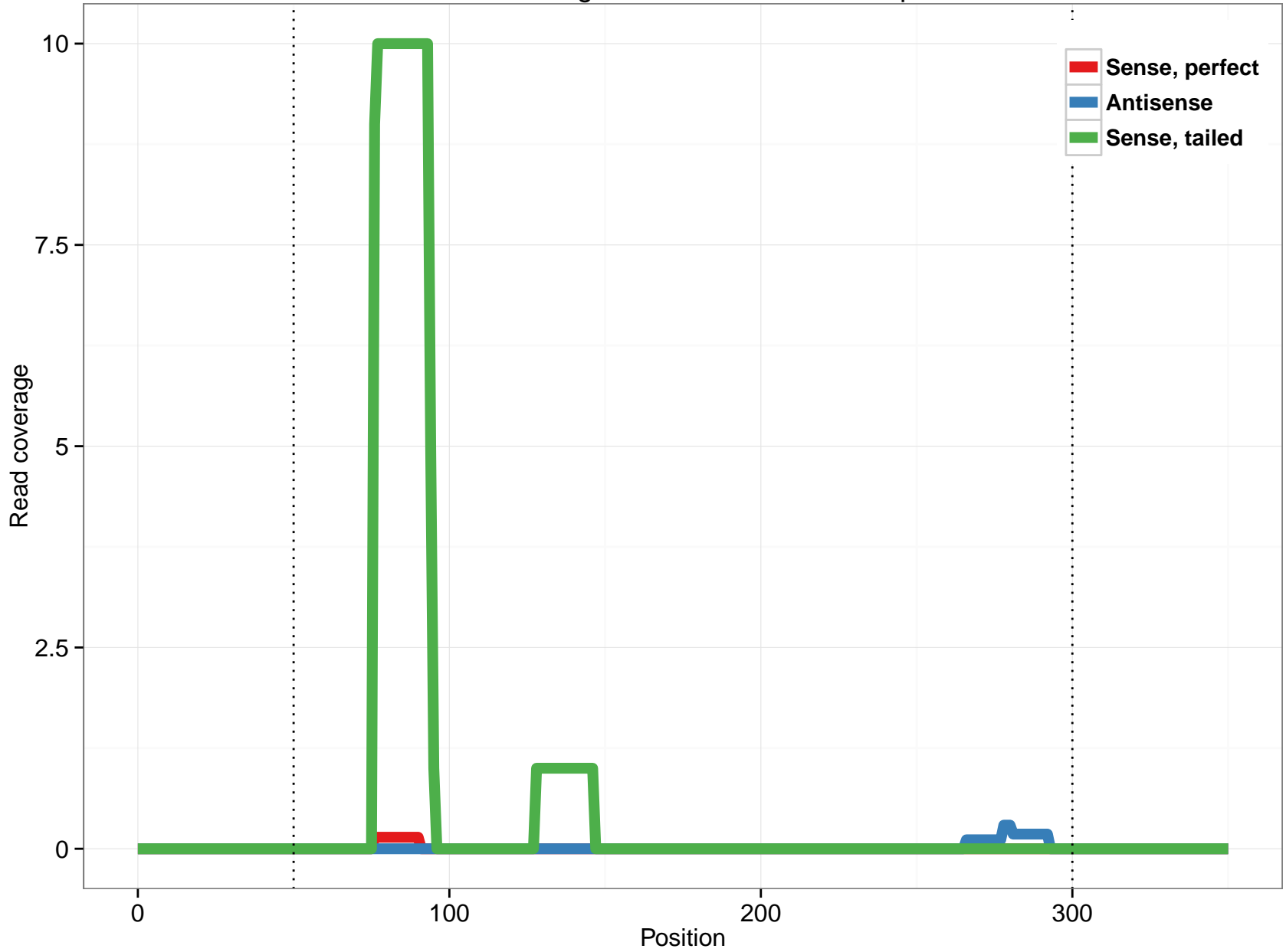
rheMac3_genscan_chr10.1875_3.5p
