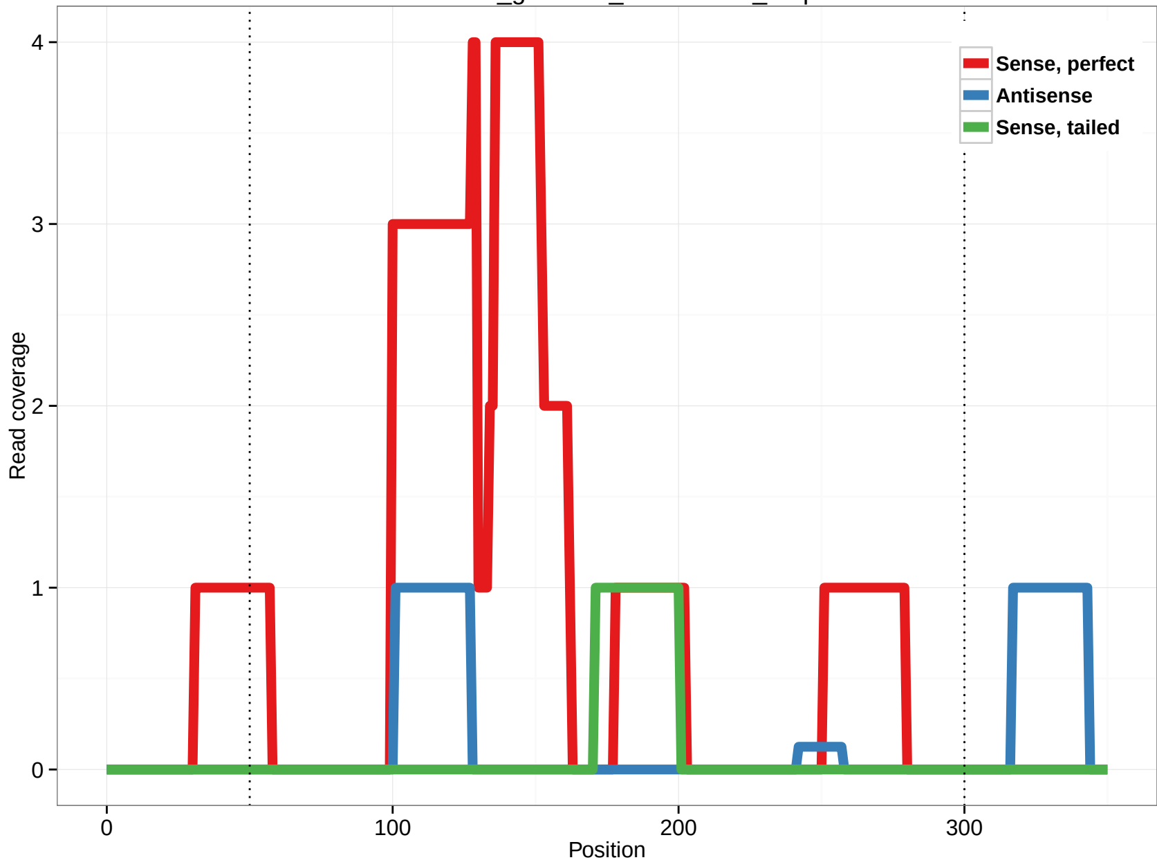
rheMac3_genscan_chr10.1870_8.5p
