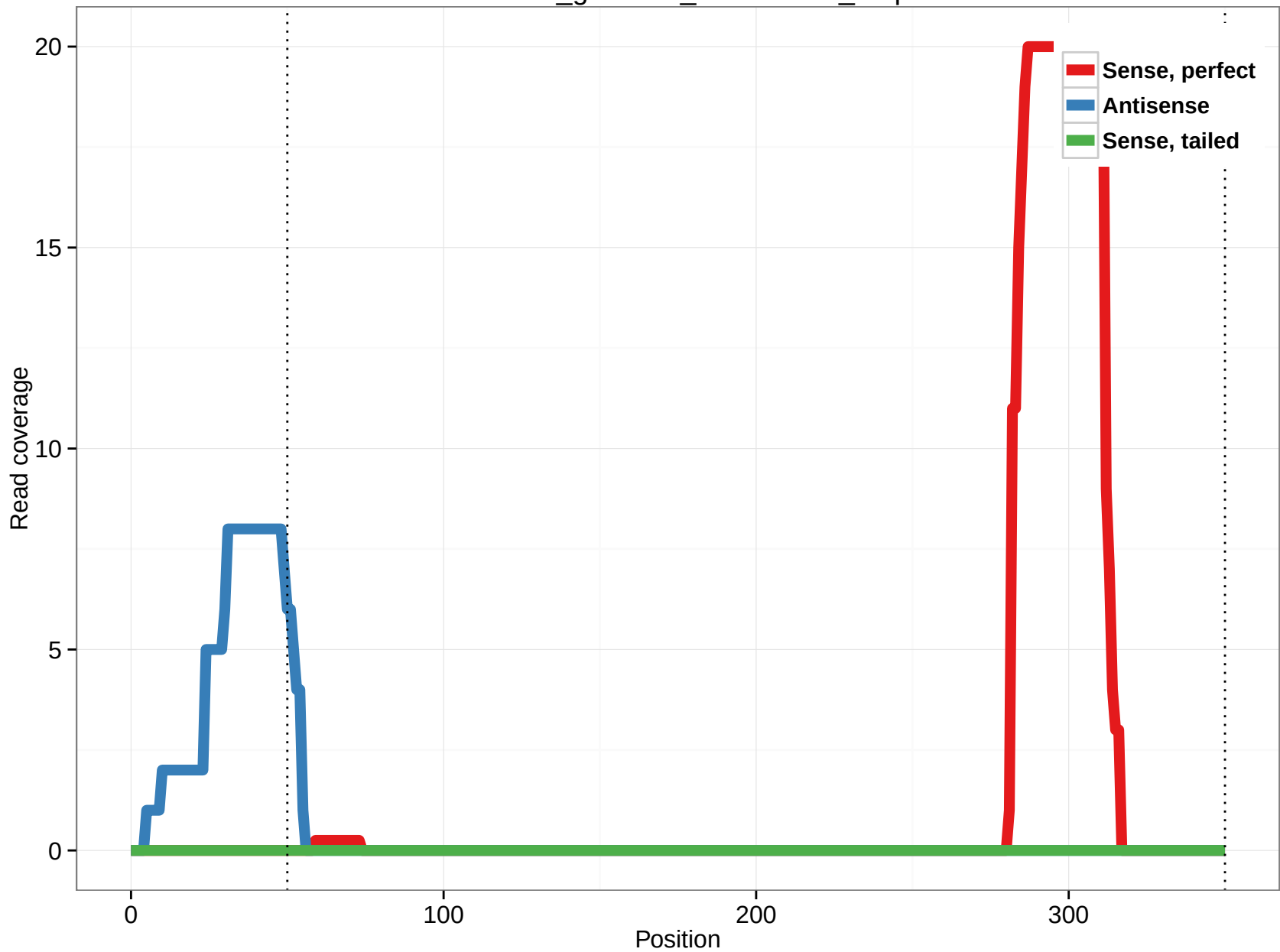
rheMac3_genscan_chr10.1858_1.5p
