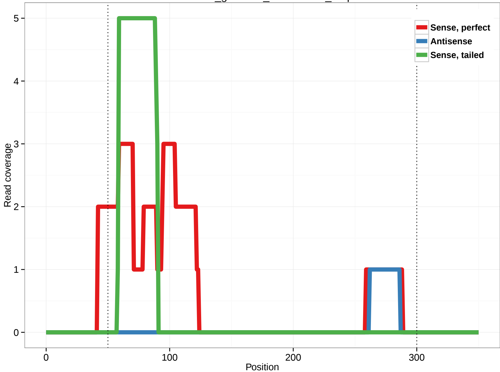
rheMac3_genscan_chr10.1858_0.3p
