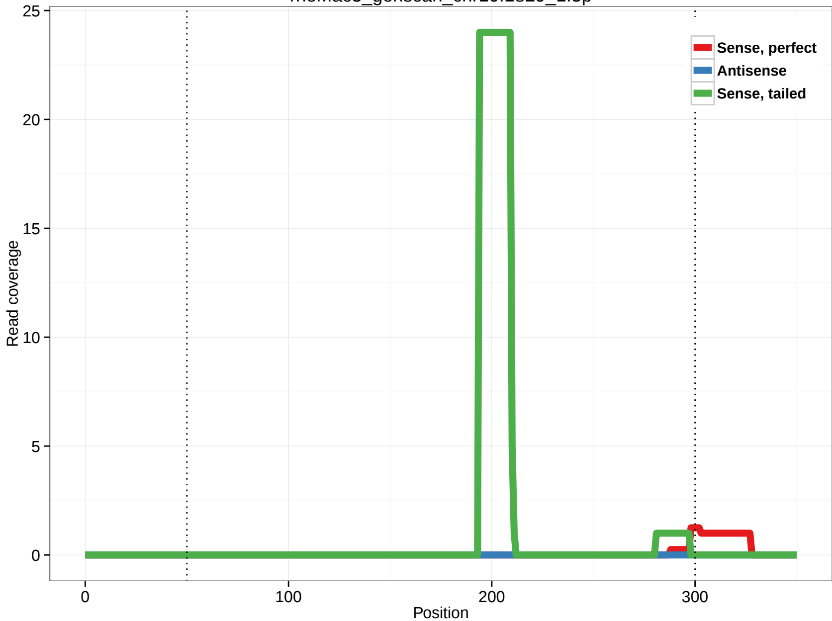
rheMac3_genscan_chr10.1829_1.5p
