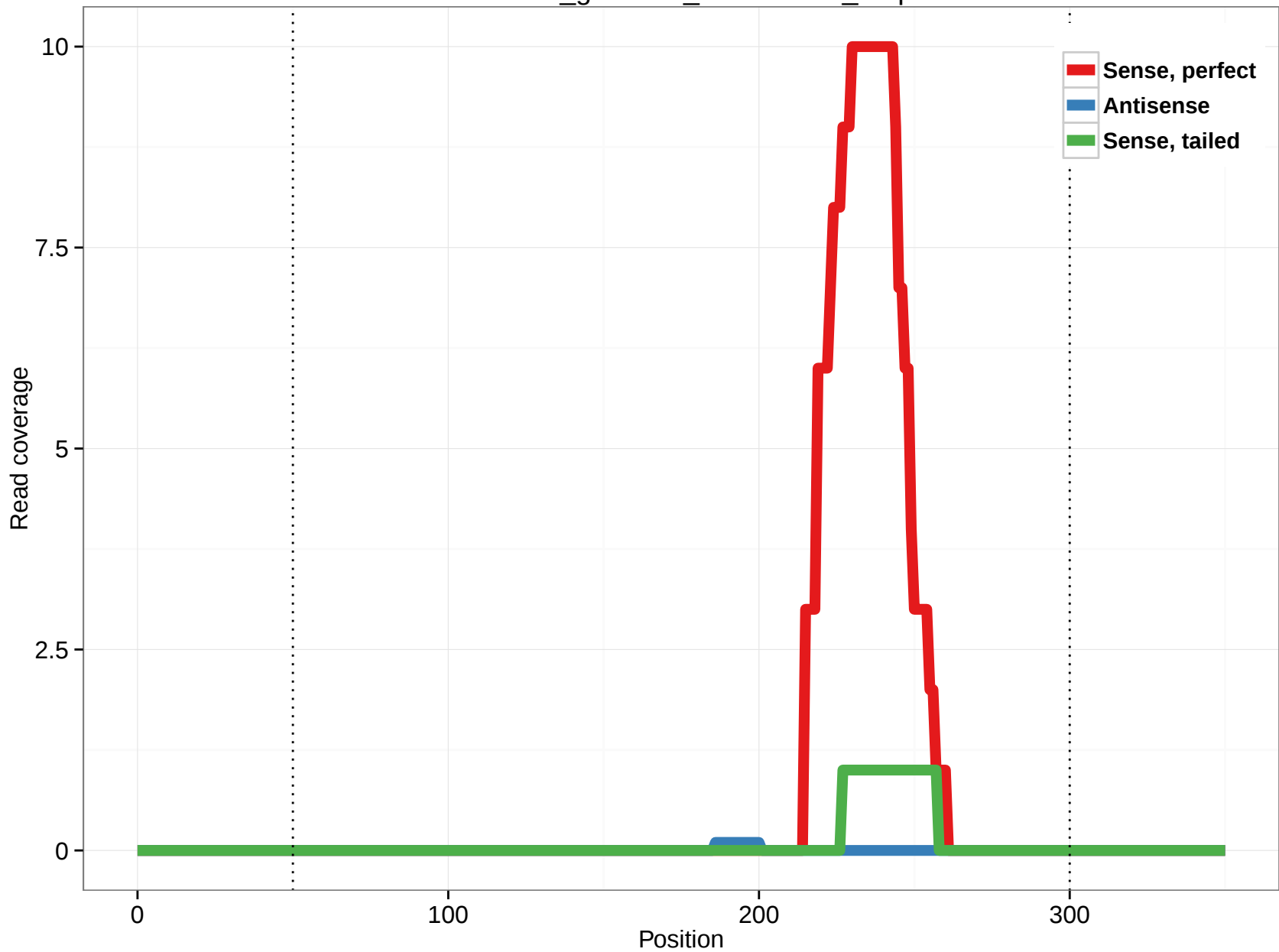
rheMac3_genscan_chr10.1778_3.3p
