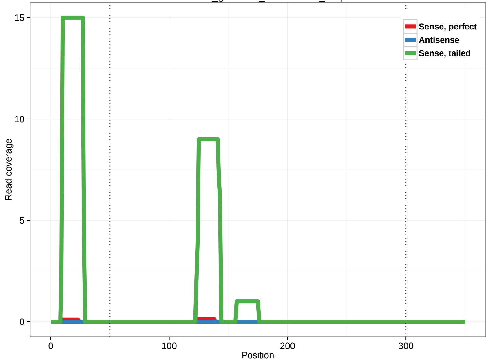
rheMac3_genscan_chr10.1748_1.3p
