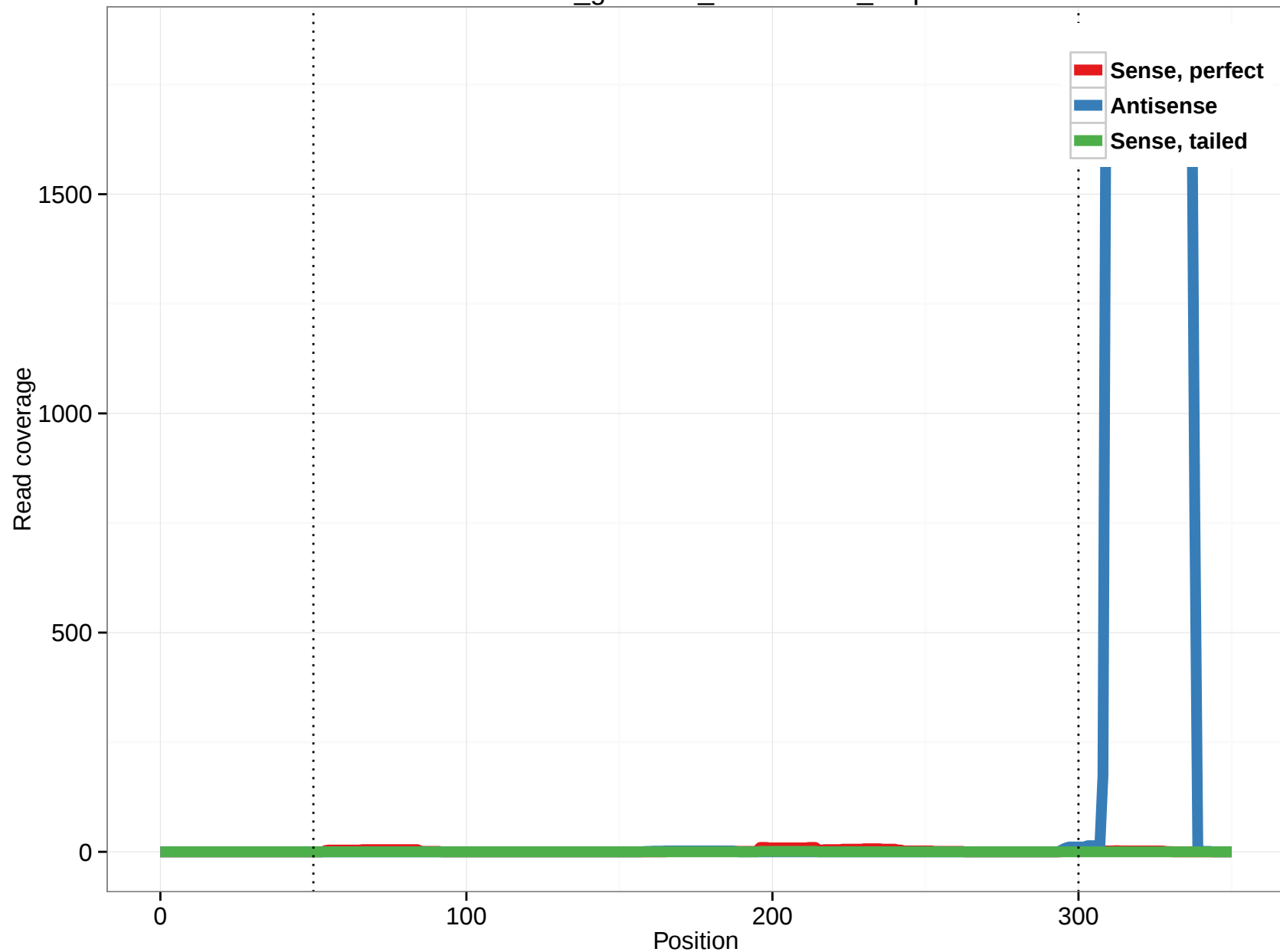
rheMac3_genscan_chr10.1732_2.3p
