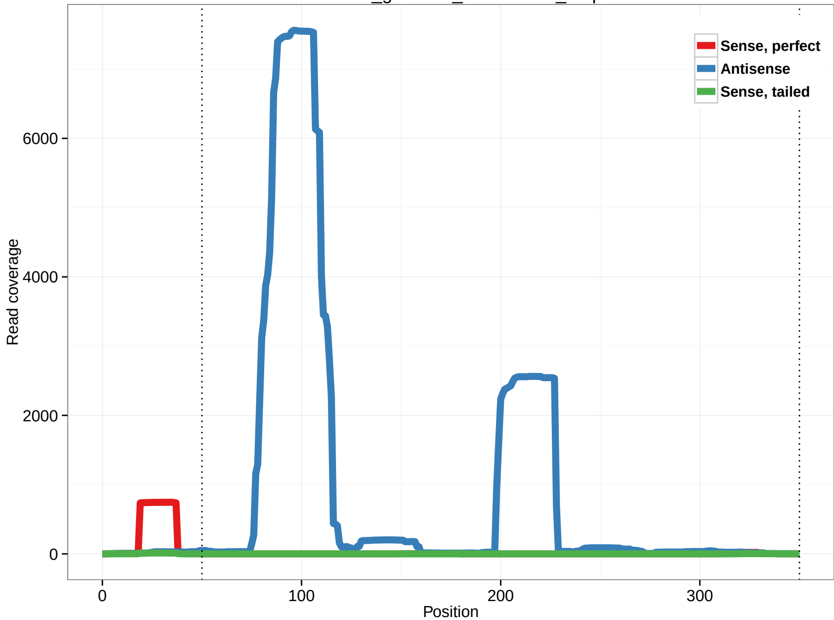
rheMac3_genscan_chr10.1731_5.5p
