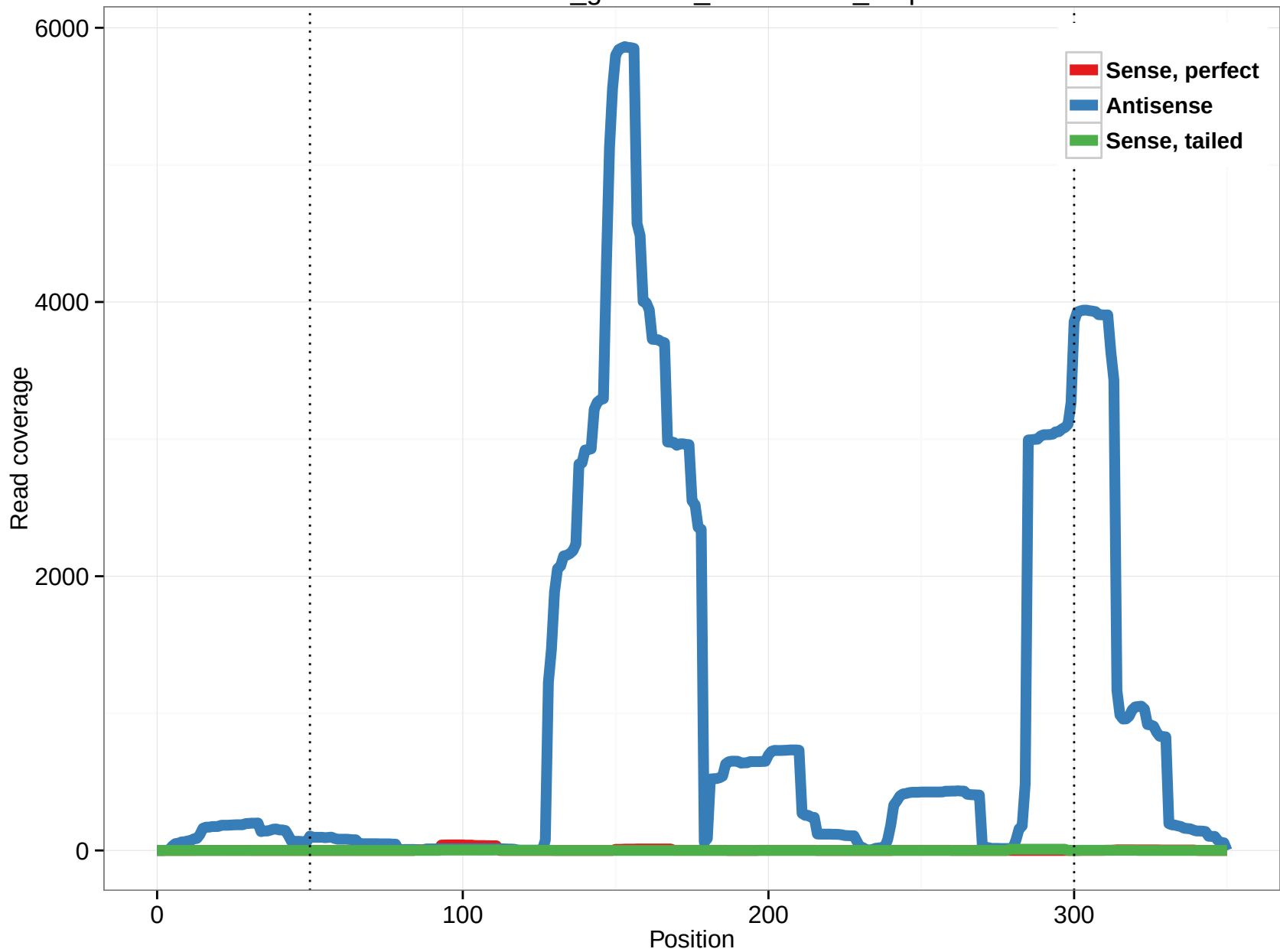
rheMac3_genscan_chr10.1731_2.3p
