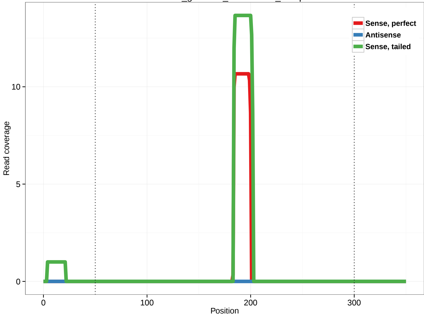
rheMac3_genscan_chr10.1713_14.3p
