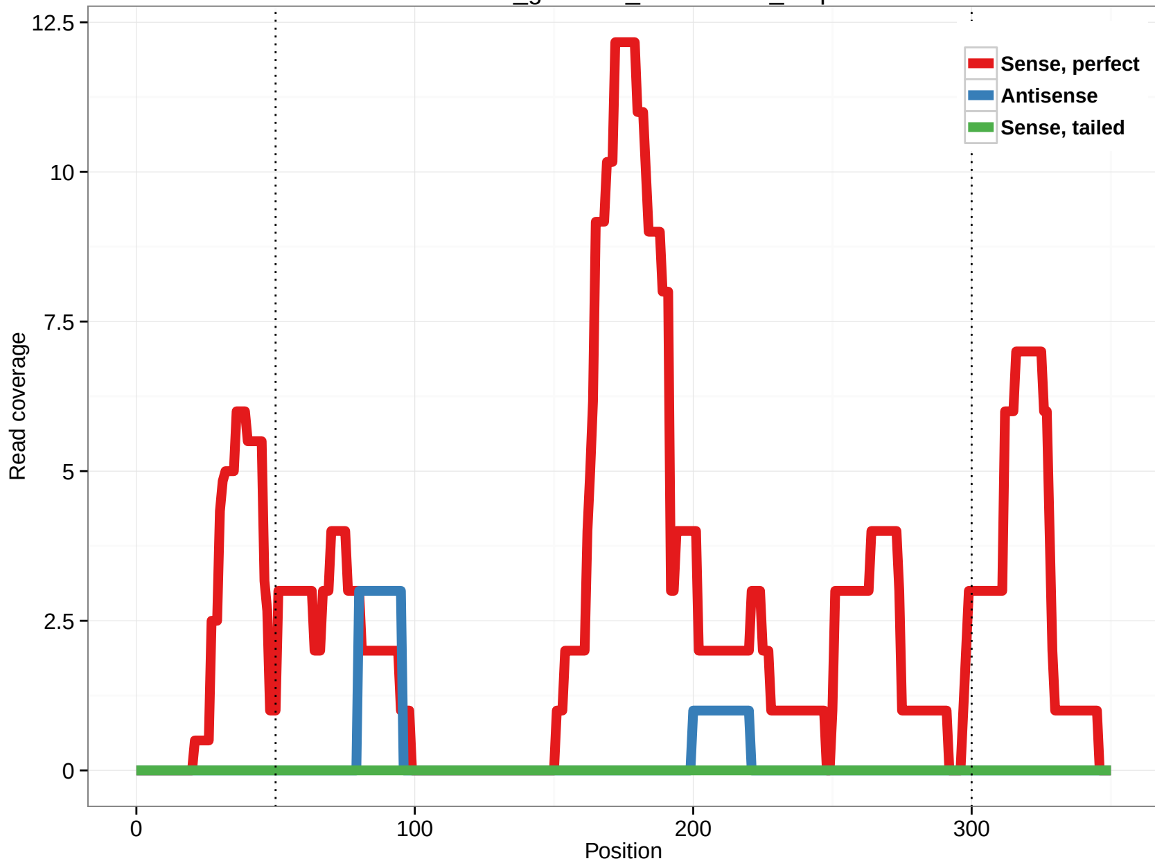
rheMac3_genscan_chr10.1698_0.5p
