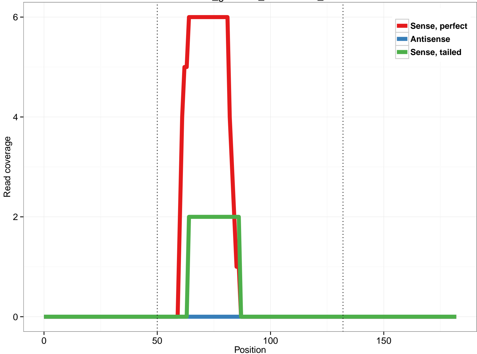
rheMac3_genscan_chr10.1690_7
