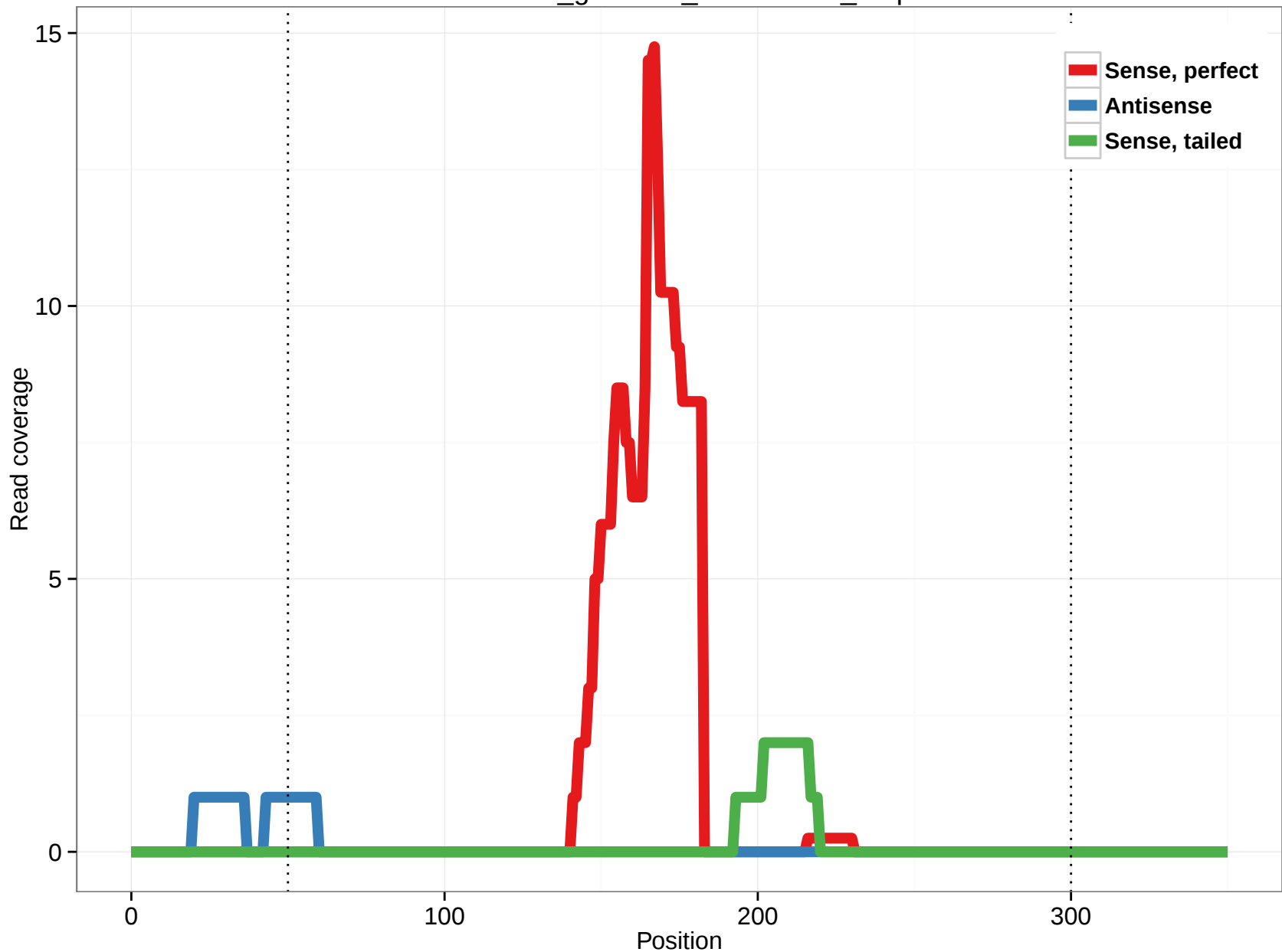
rheMac3_genscan_chr10.1661_9.3p
