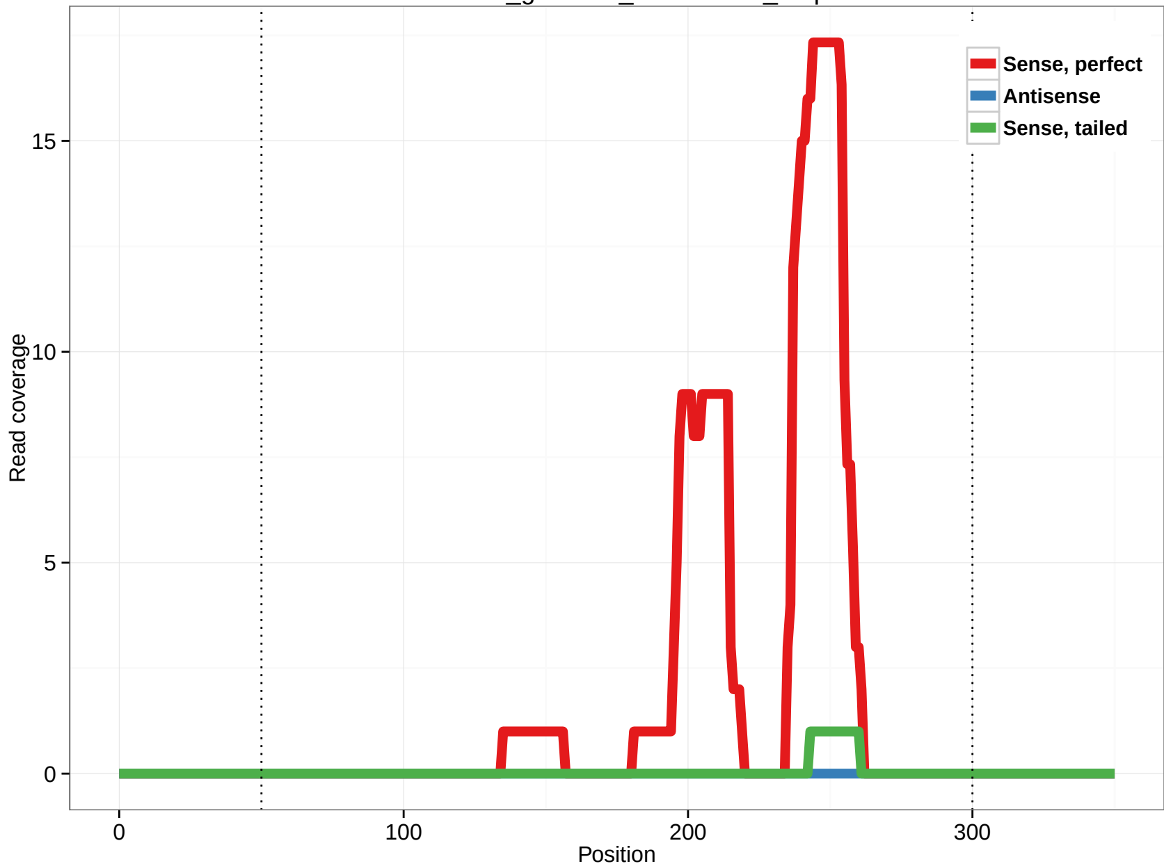
rheMac3_genscan_chr10.1661_0.5p
