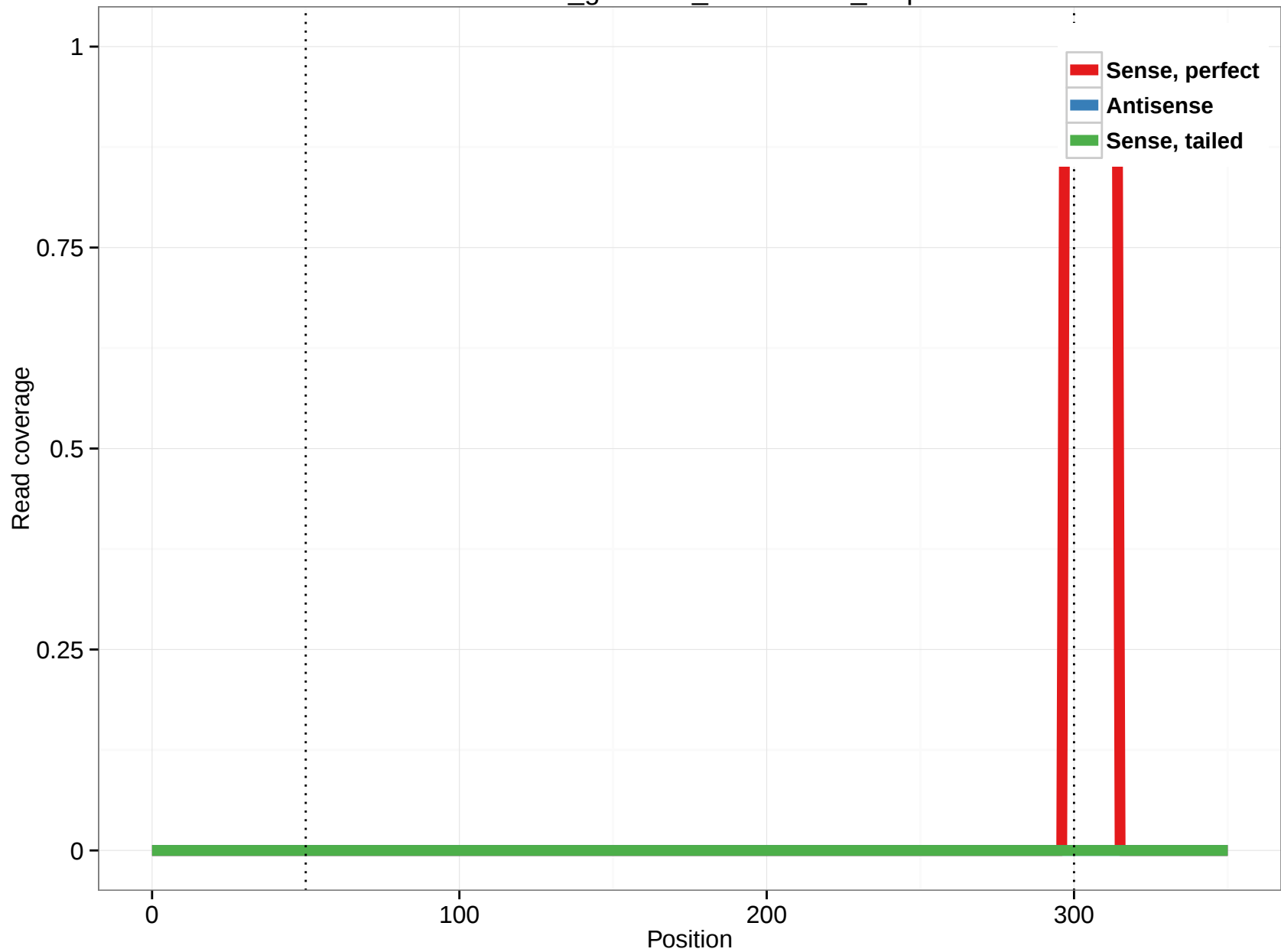
rheMac3_genscan_chr10.1654_3.3p
