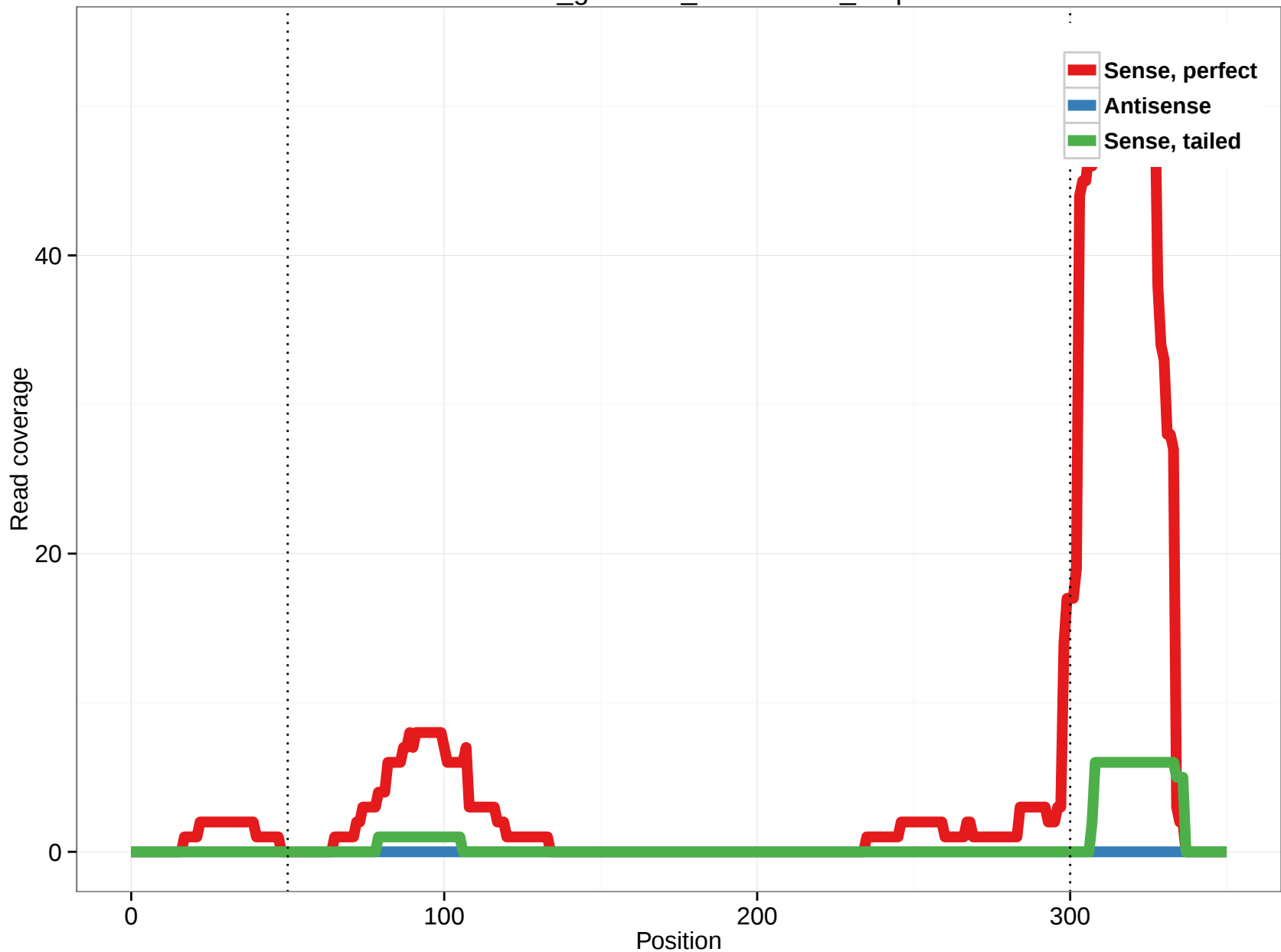
rheMac3_genscan_chr10.1653_2.5p
