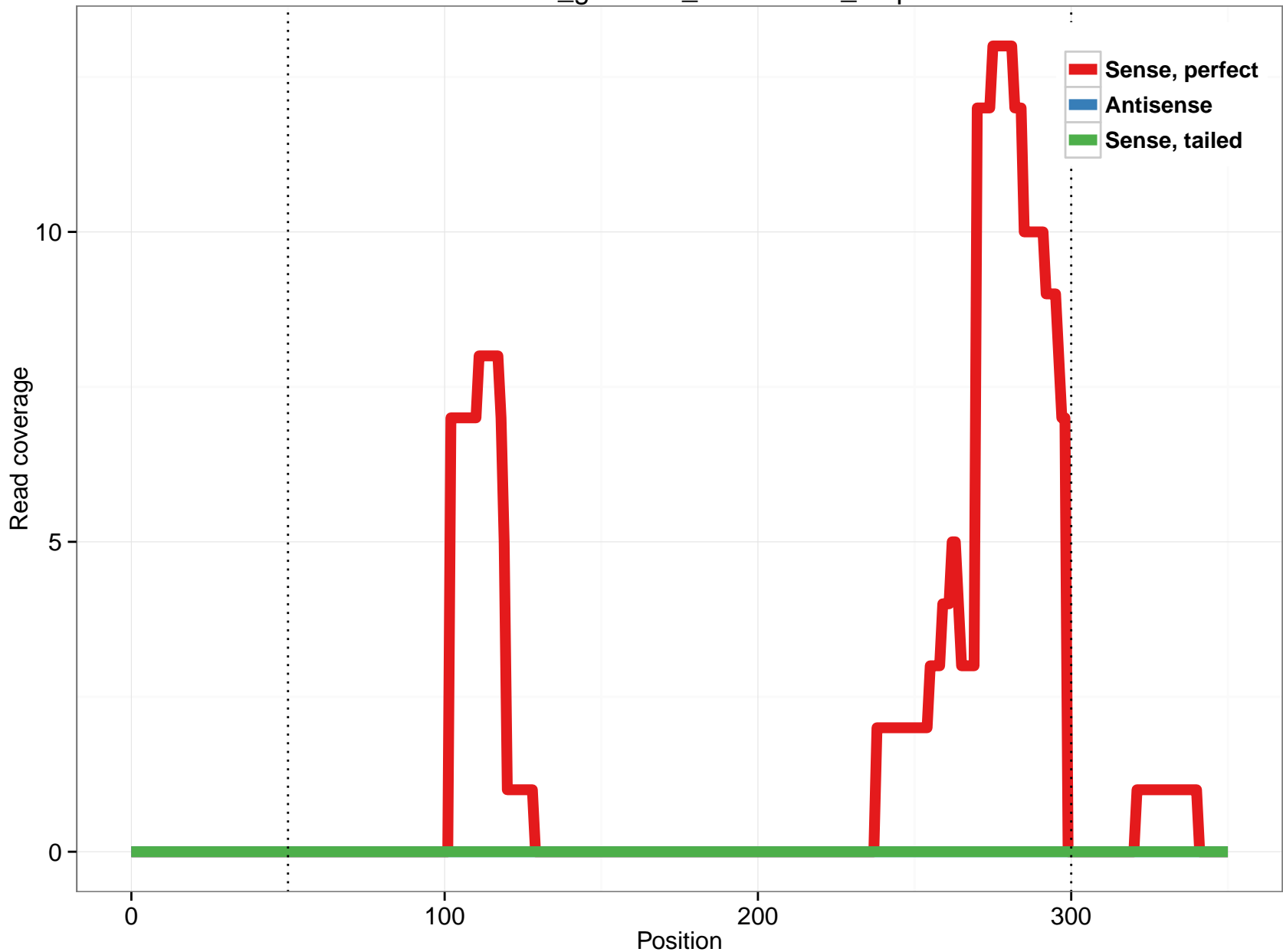
rheMac3_genscan_chr10.1653_0.5p
