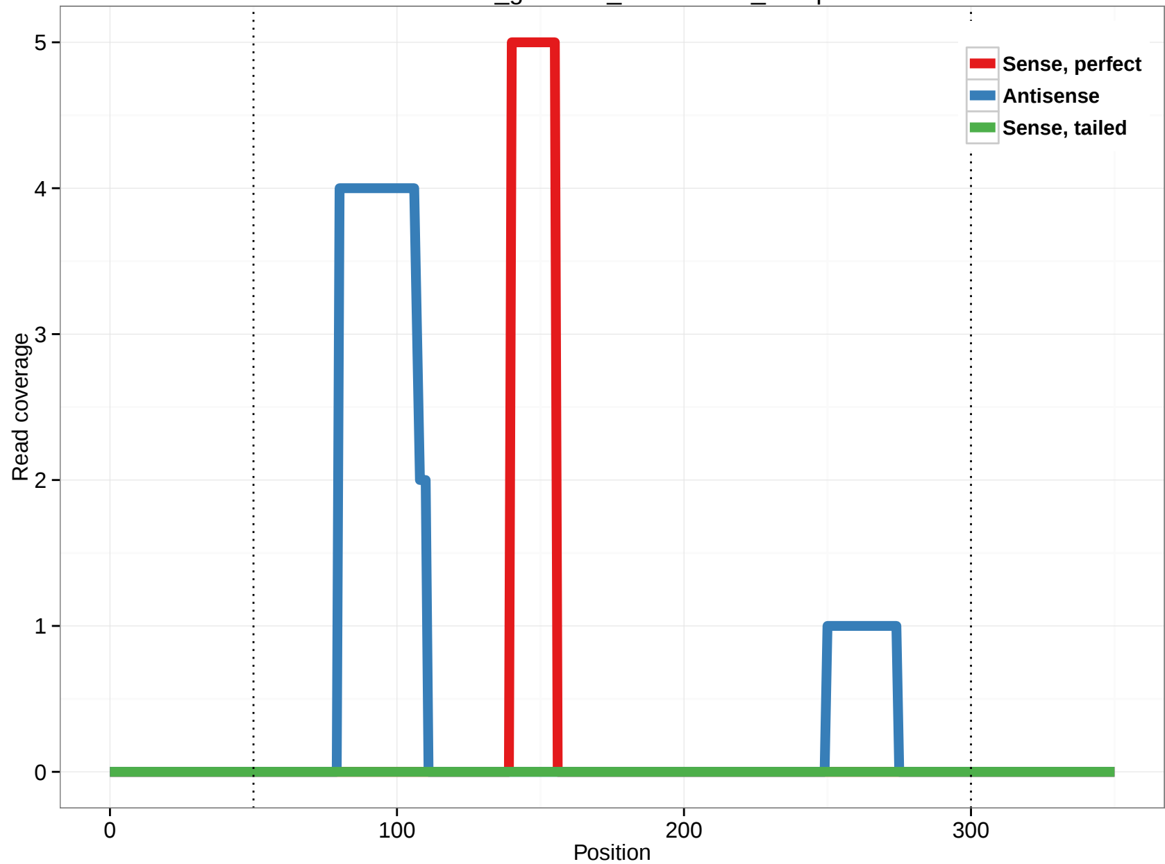
rheMac3_genscan_chr10.1639_23.3p
